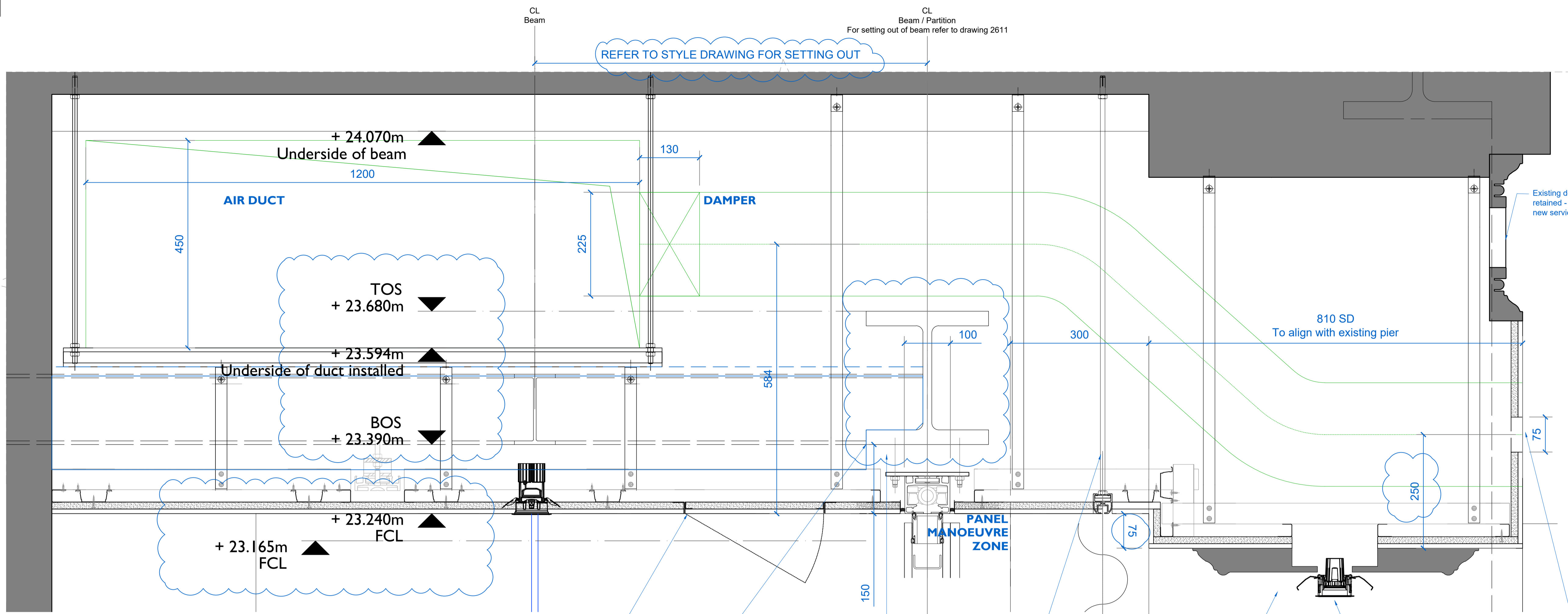
1 EVENT SPACE FOLDING PARTITION HEAD DETAIL 6006 1:5
