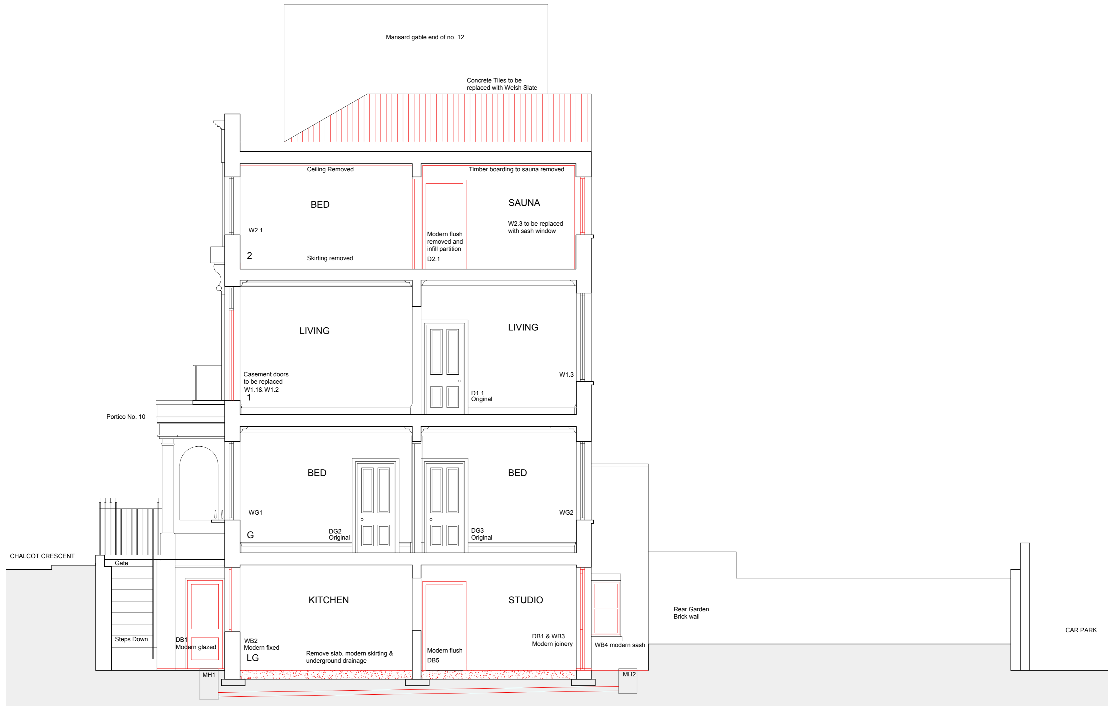
EXISTING SECTION BB
