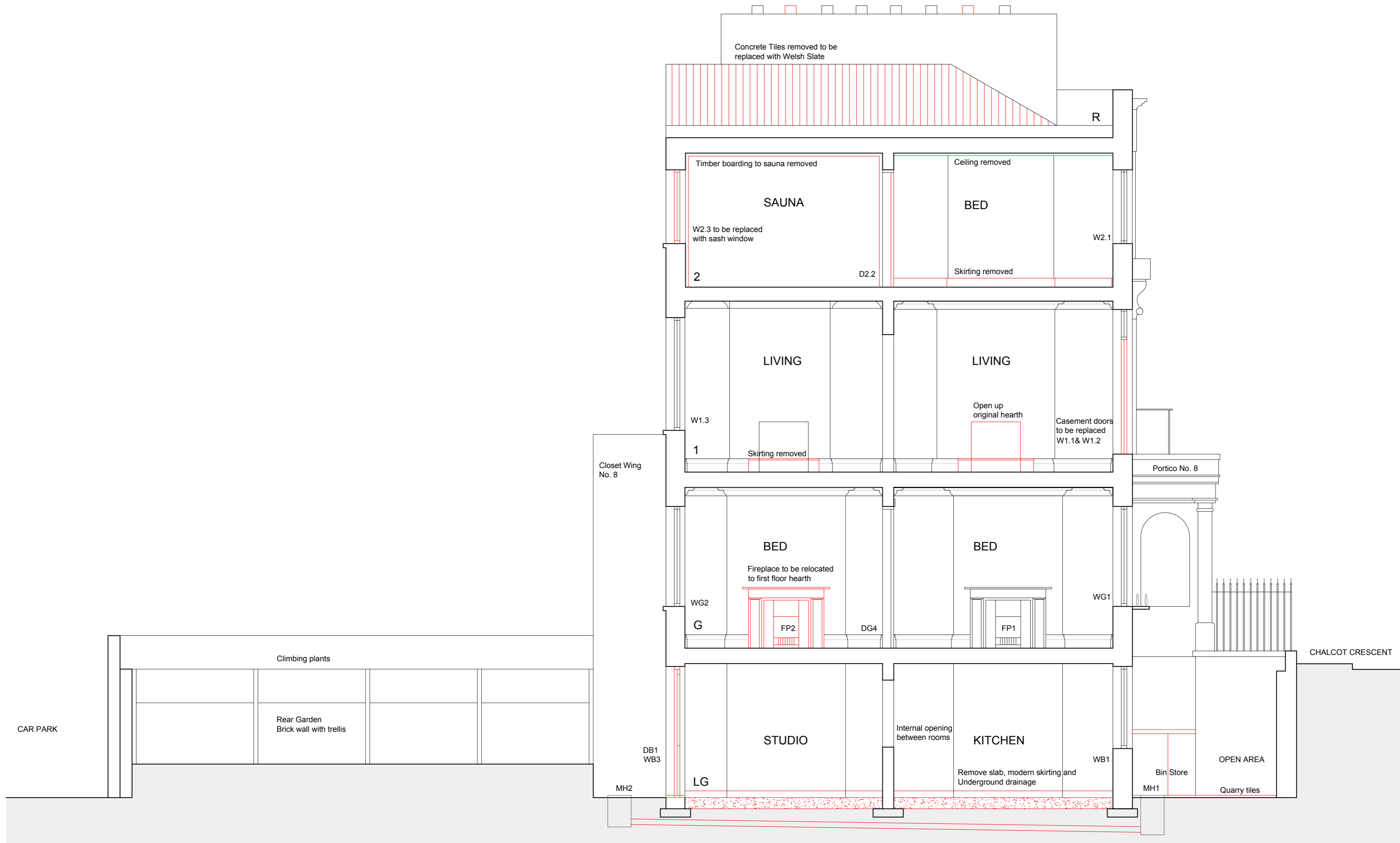
EXISTING SECTION AA
