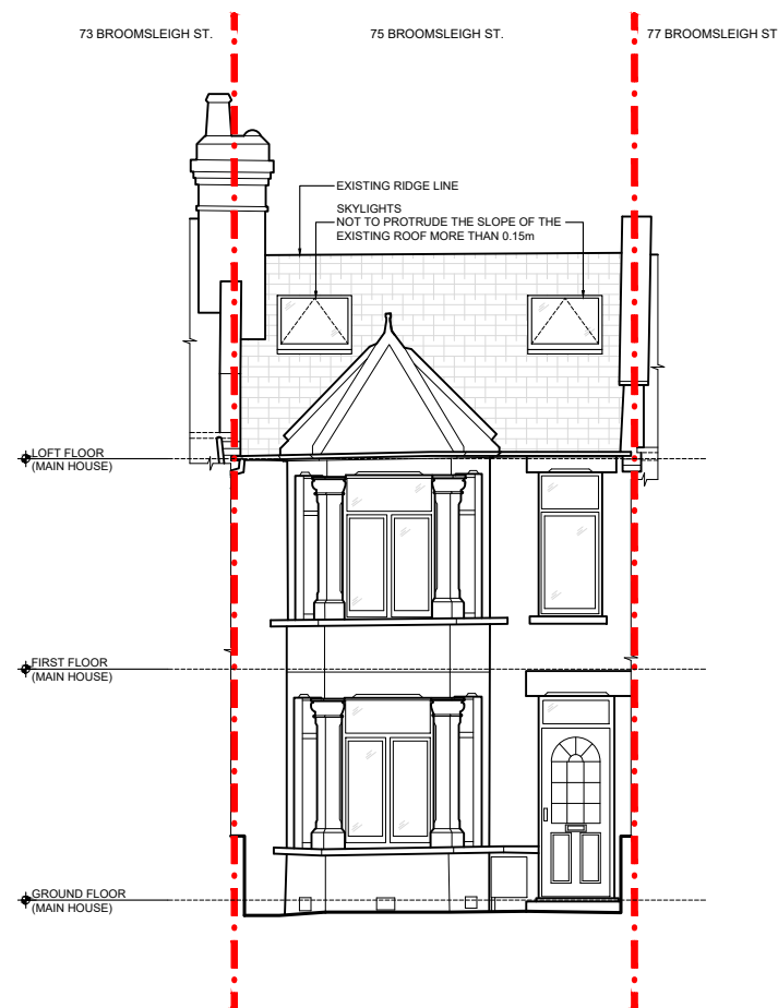
② Proposed Front Elevation
