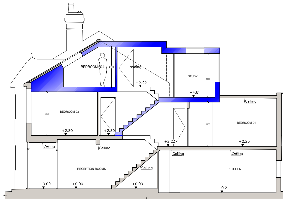
1 Proposed Section
