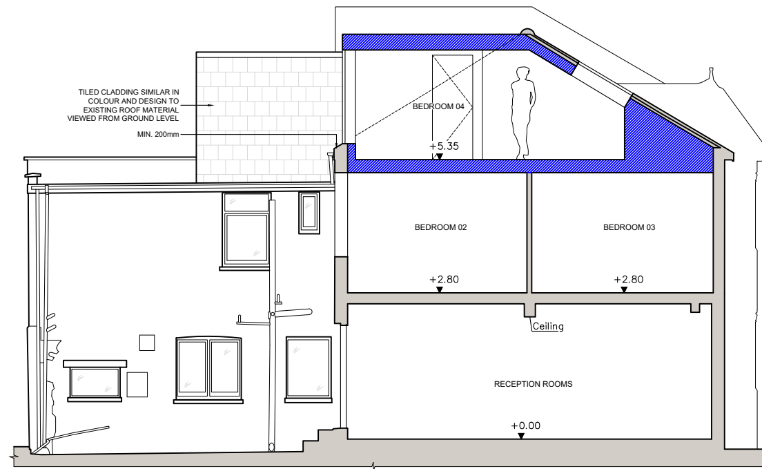
2 Proposed Section
