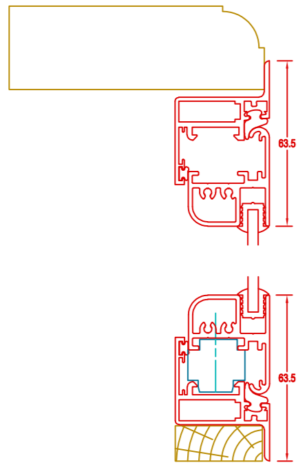
Side View 1:2
