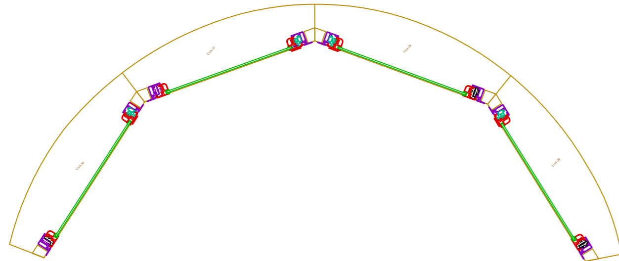
Plan View with secondary glazing 1:10
