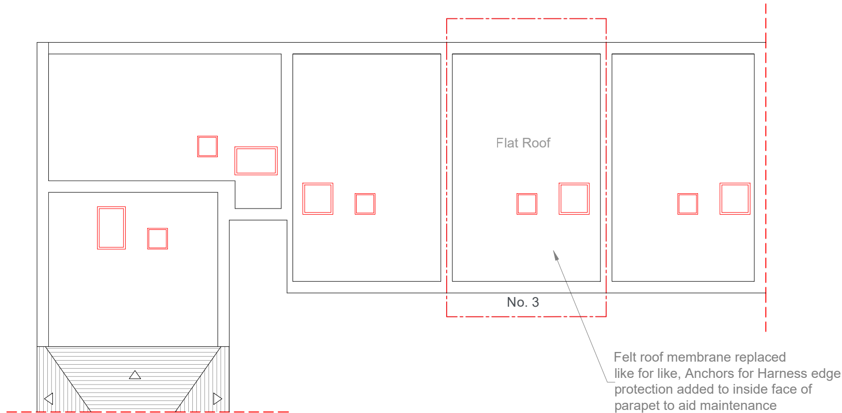
1 Proposed Roof Plan Scale: 1:100 @ A3
