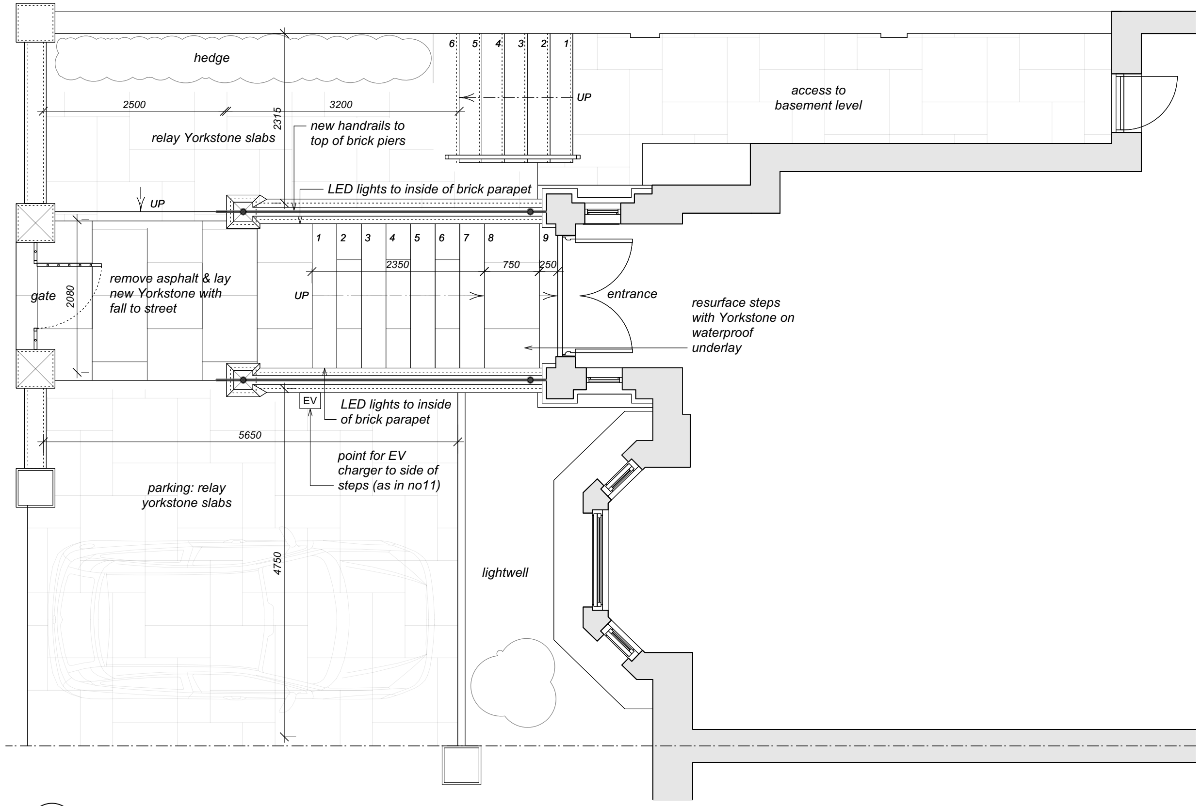
2 Proposed ground floor plan 02-01 Scale: 1:50
