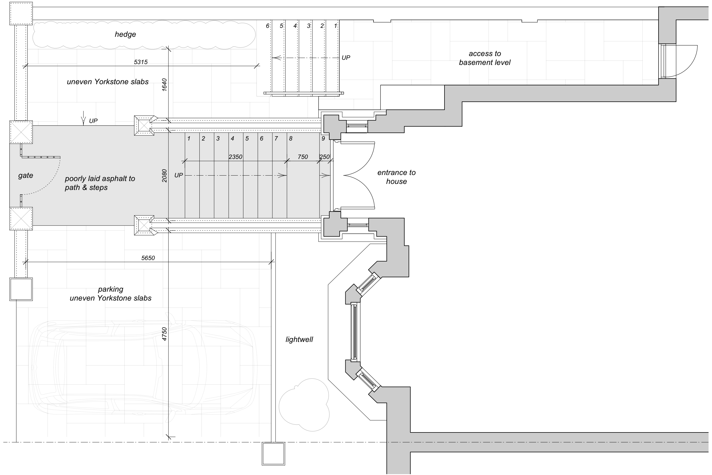
1 Existing ground floor plan 01-01 Scale: 1:50
