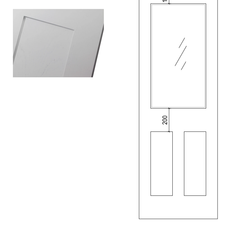
D G.01 Proposed new toilet door
