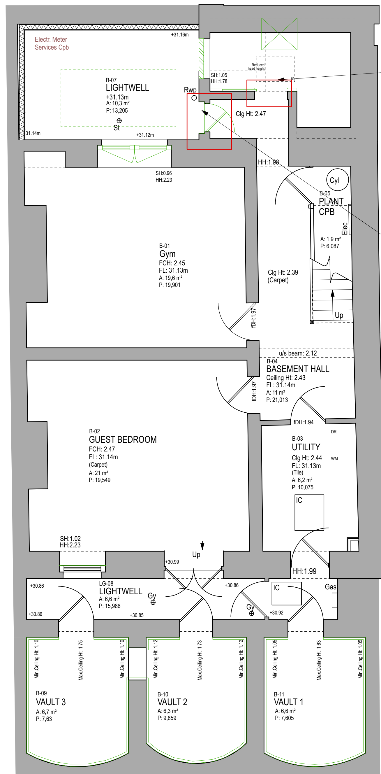
1 LOWER GROUND FLOOR 1:50
