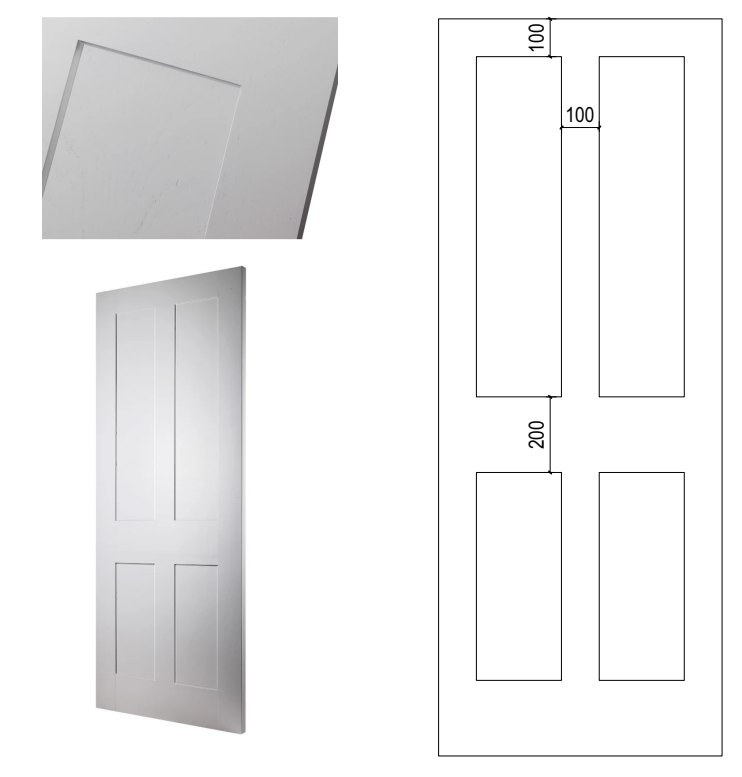
D L.01 Proposed new door to bathroom
