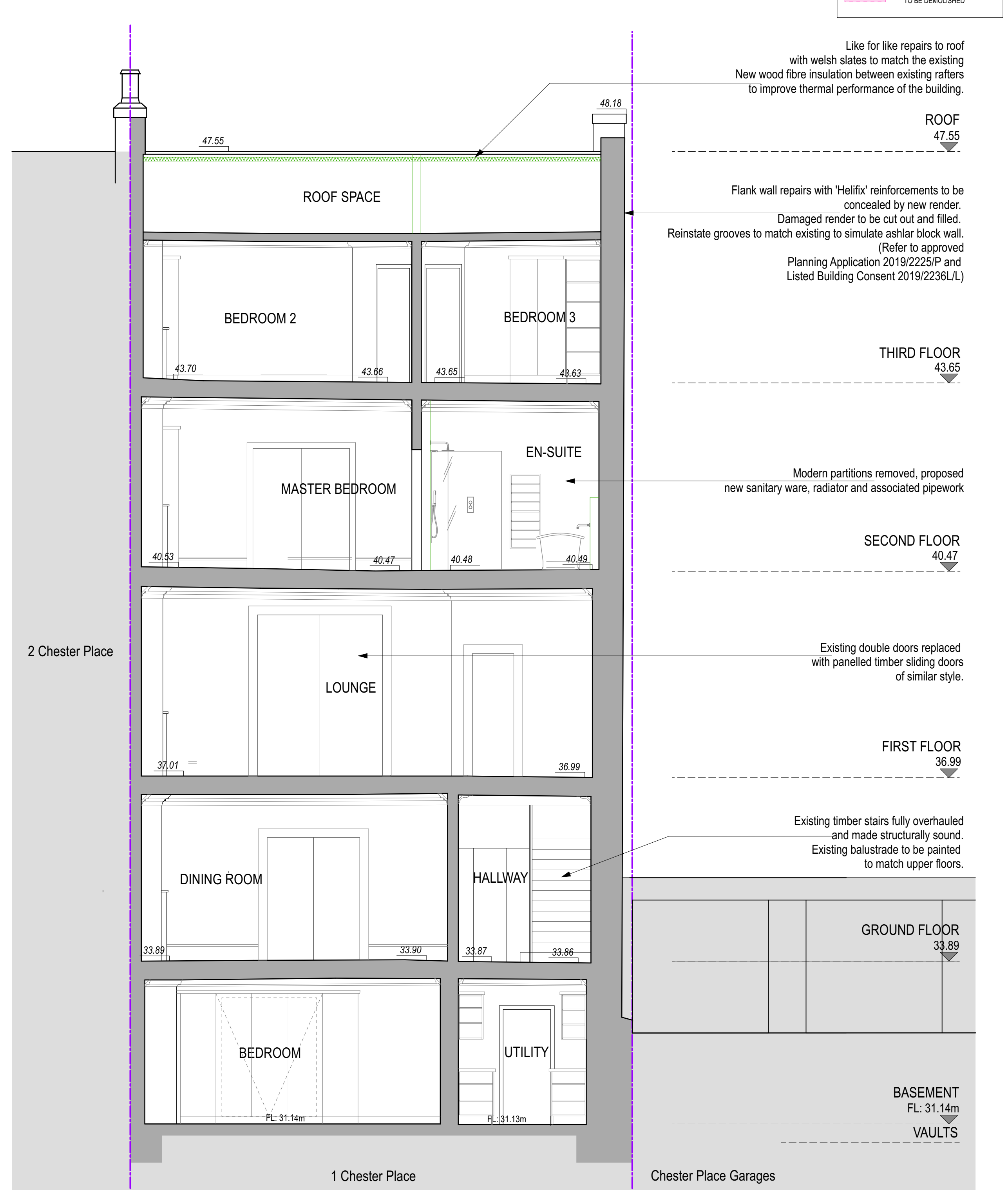
SECTION B-B ON SECTION OVERVIEW
