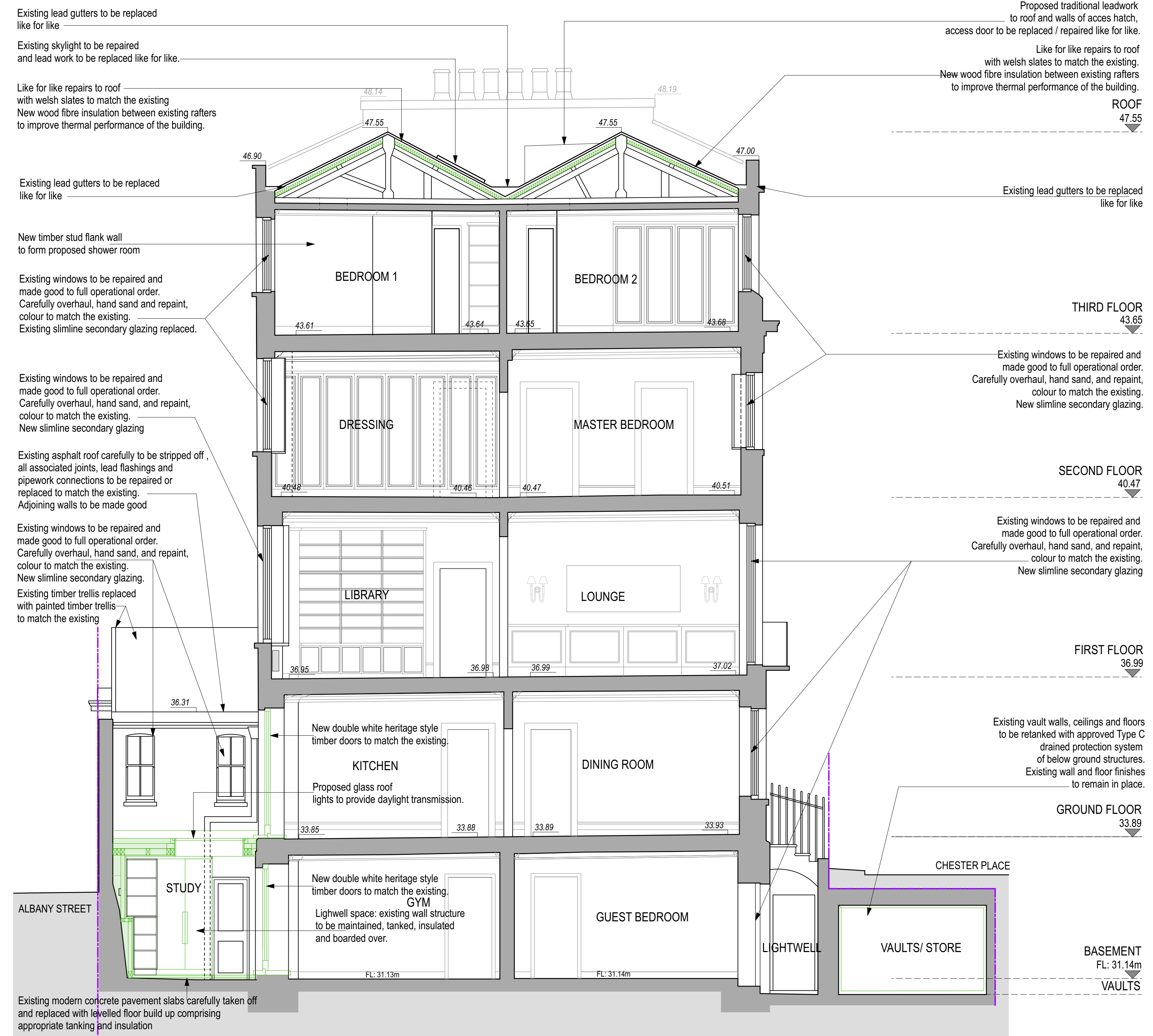
SECTION A-A ON SECTION OVERVIEW
