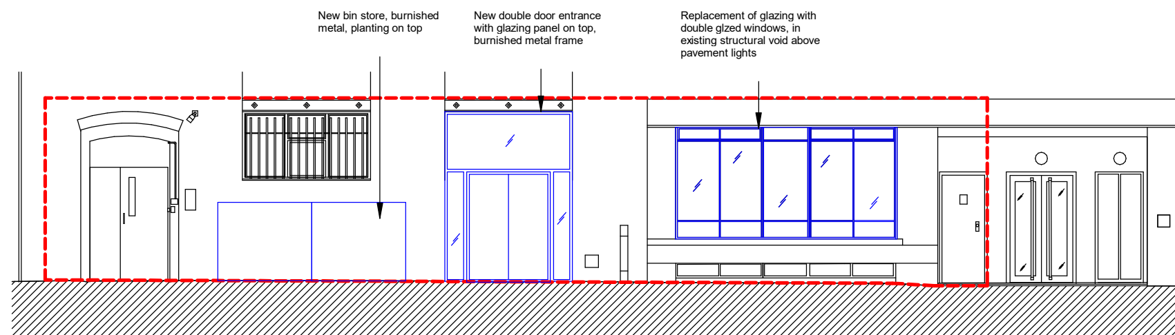
1 Proposed West Elevation - Demise 1 : 100
