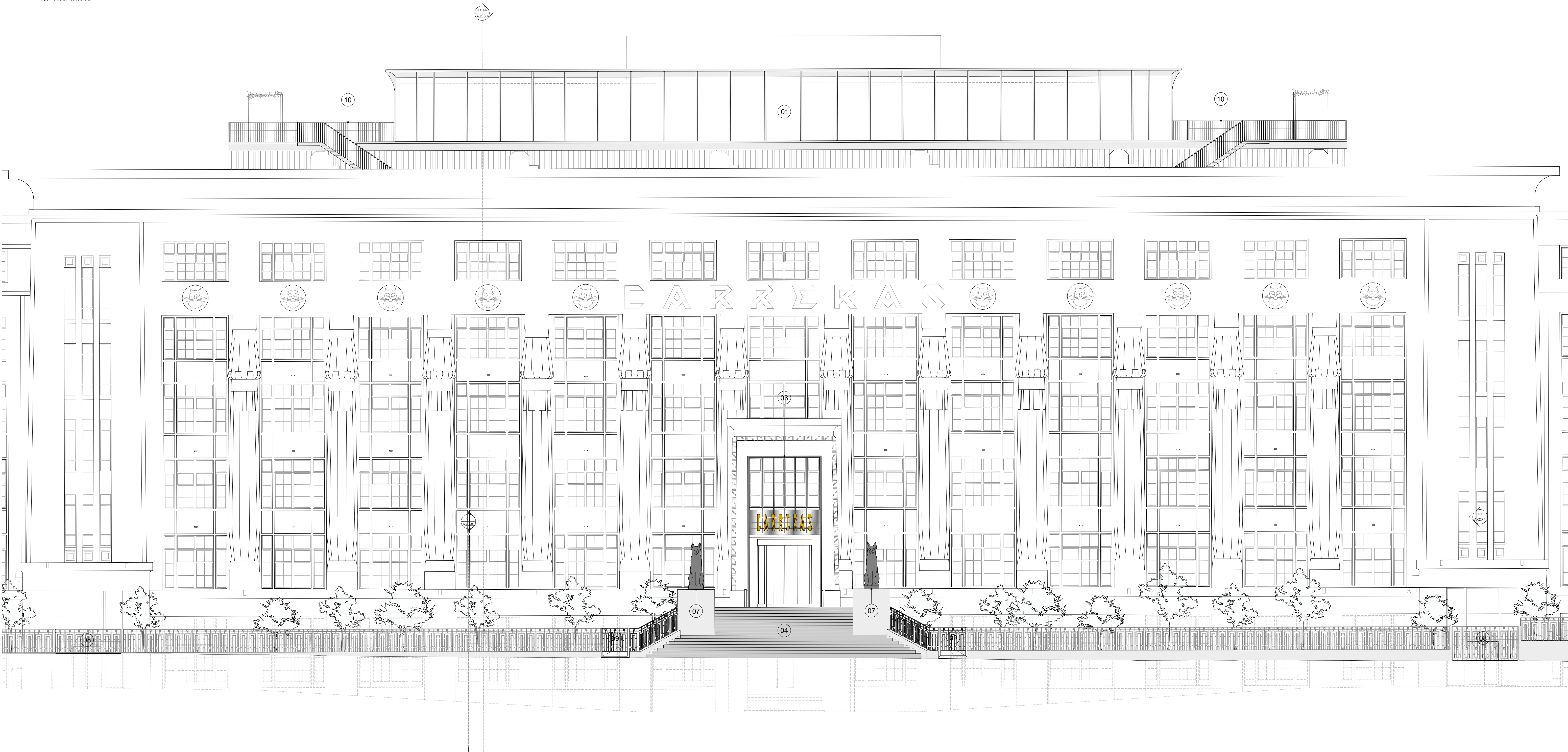
01 PROPOSED - FRONT (EAST) ELEVATION (CLOSE UP) Scale 1:100 @A1
