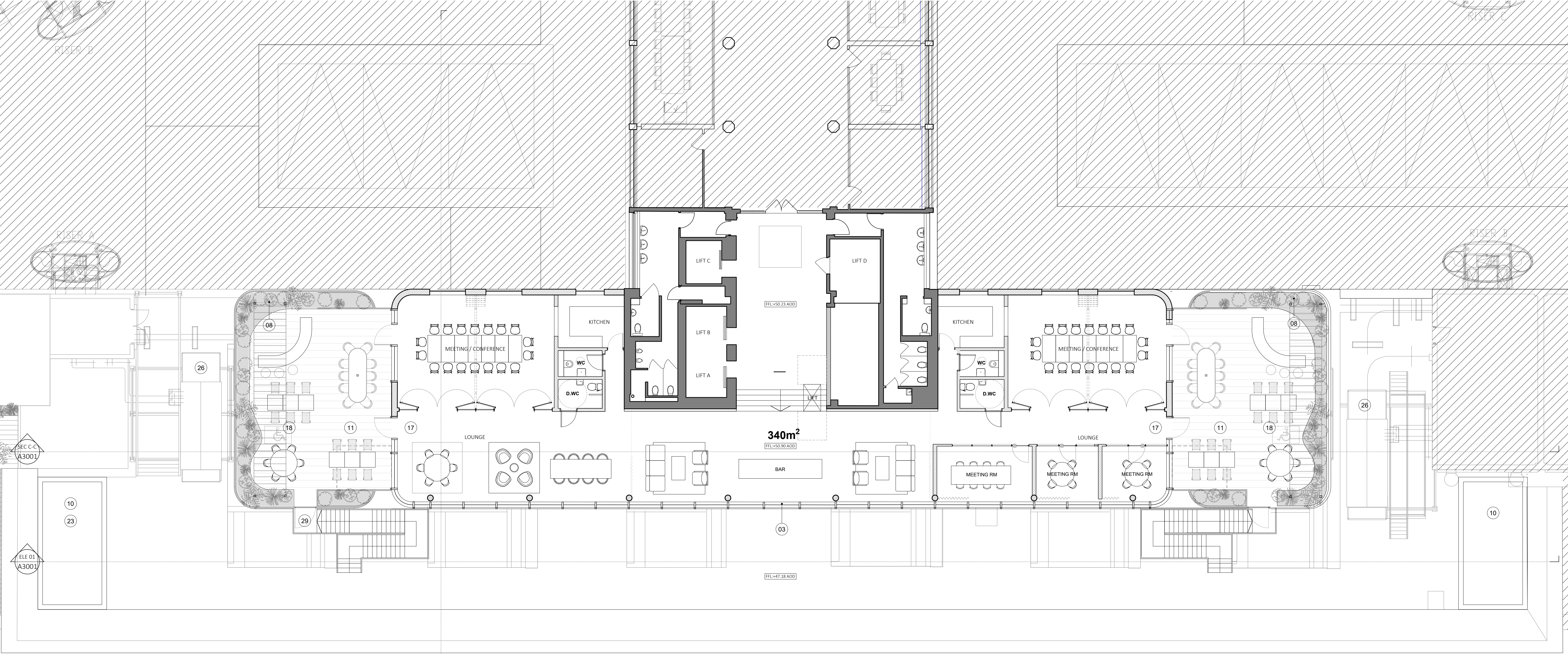
01 PROPOSED SIXTH FLOOR PAVILION DETAILED PLAN 1:100 @ A1
