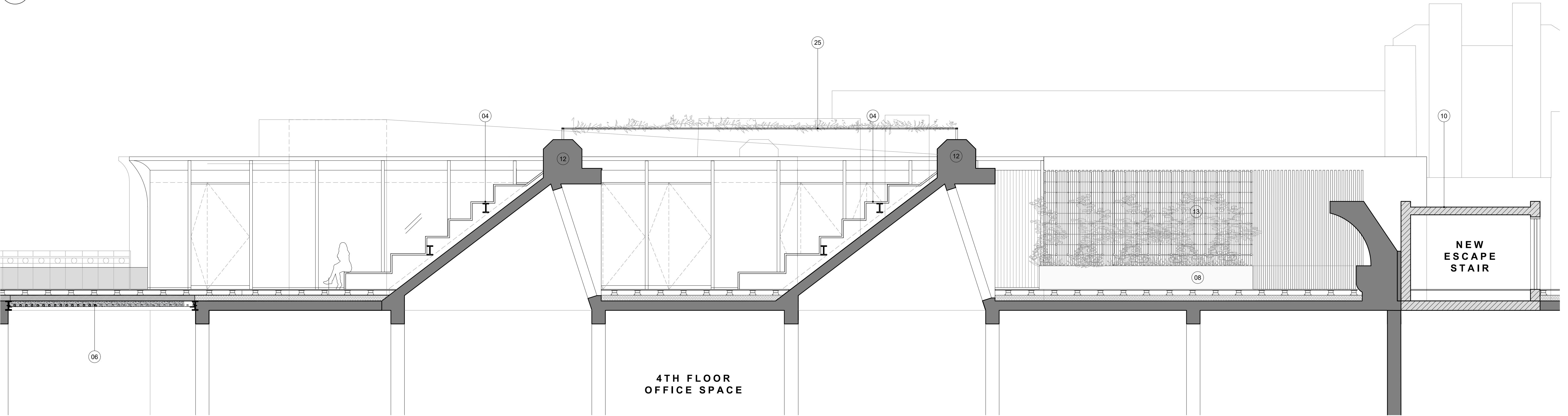
02 PROPOSED FIFTH FLOOR PAVILION SECTION F-F 1:50 @ A1
