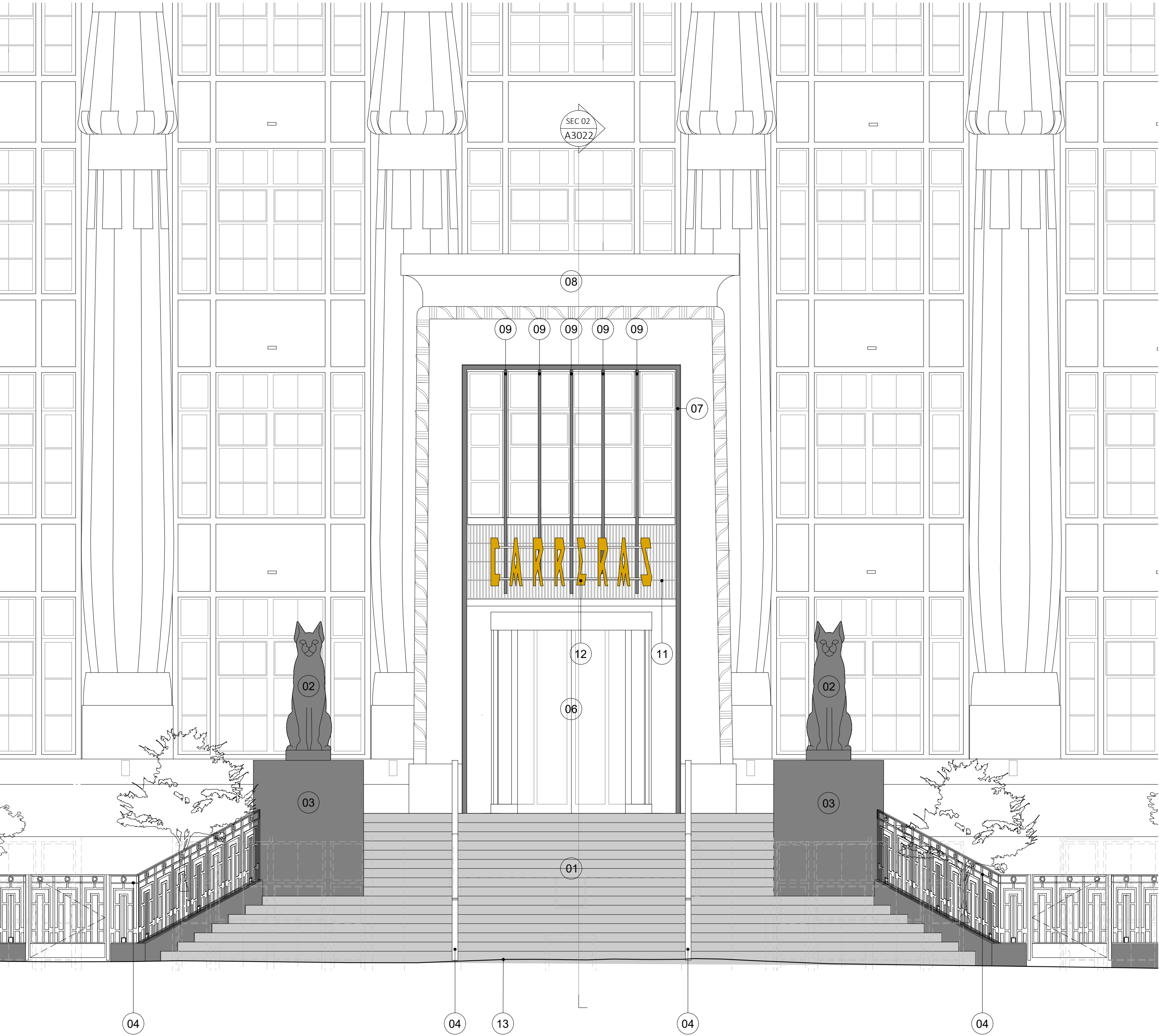
02 PROPOSED PORTAL & STAIR ELEVATION Scale 1:50 @A1
