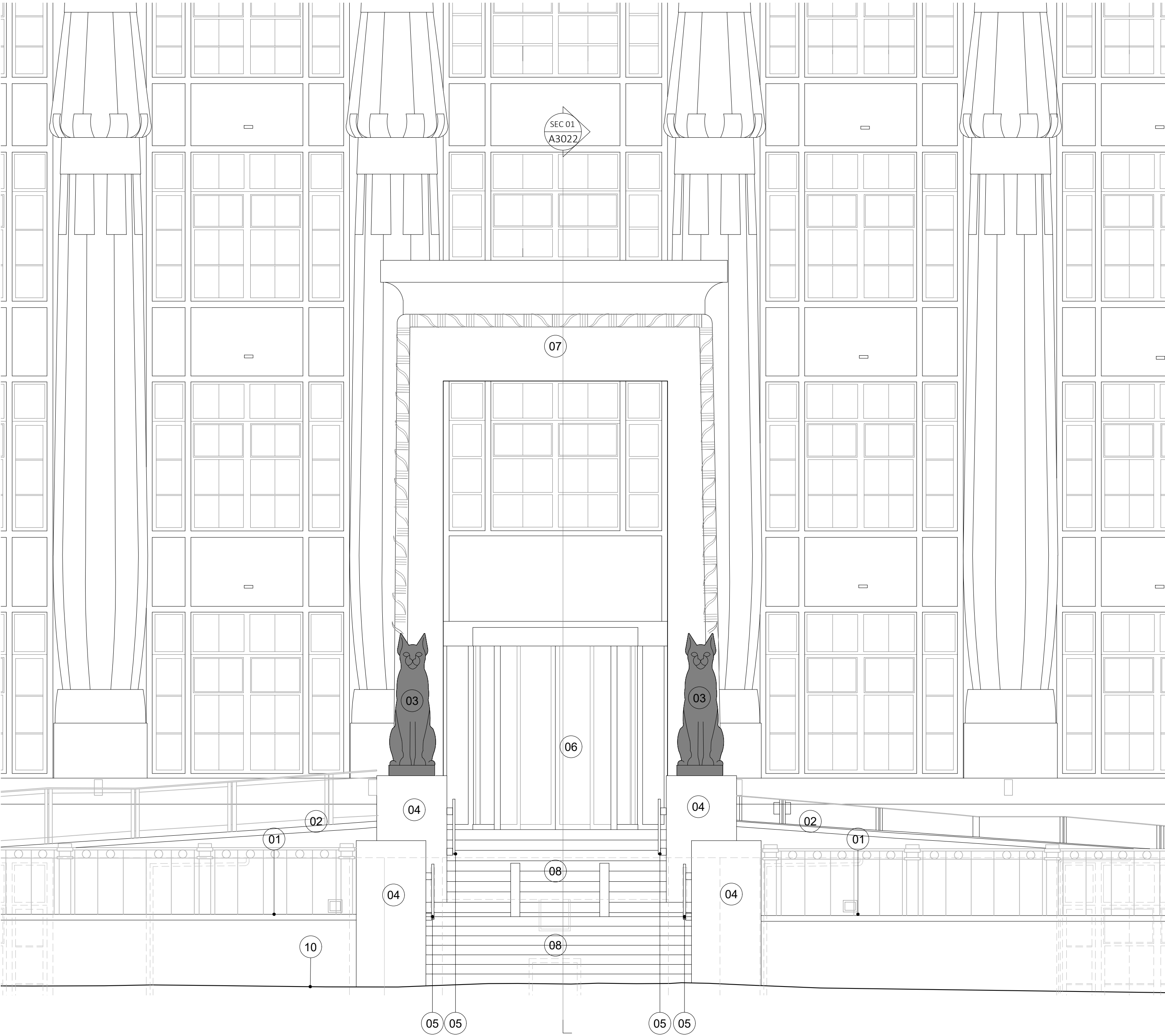
01 EXISTING PORTAL & STAIR ELEVATION Scale 1:50 @A1
