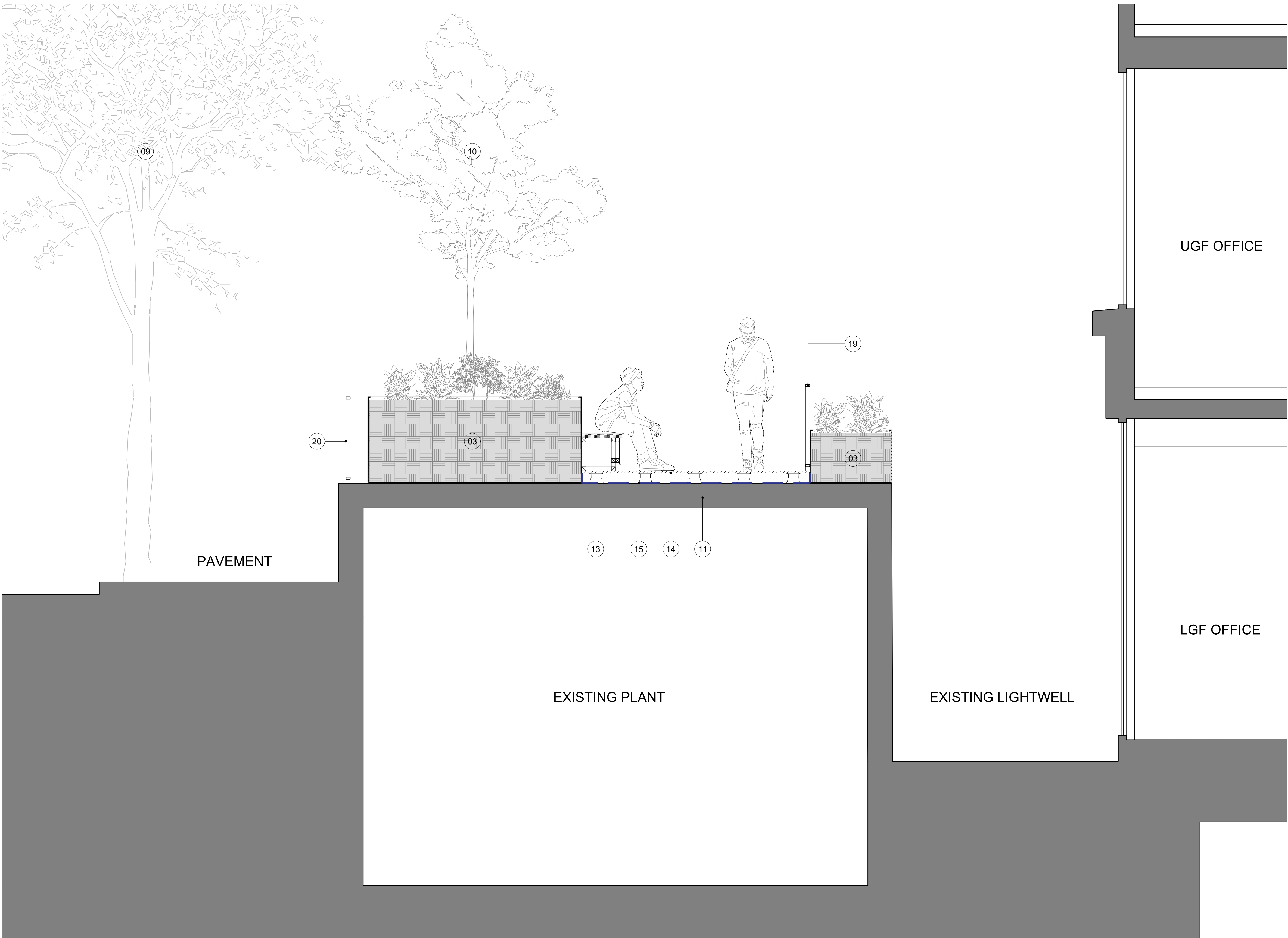
01 FRONT LANDSCAPING SECTION 02 1:25 @ A1
