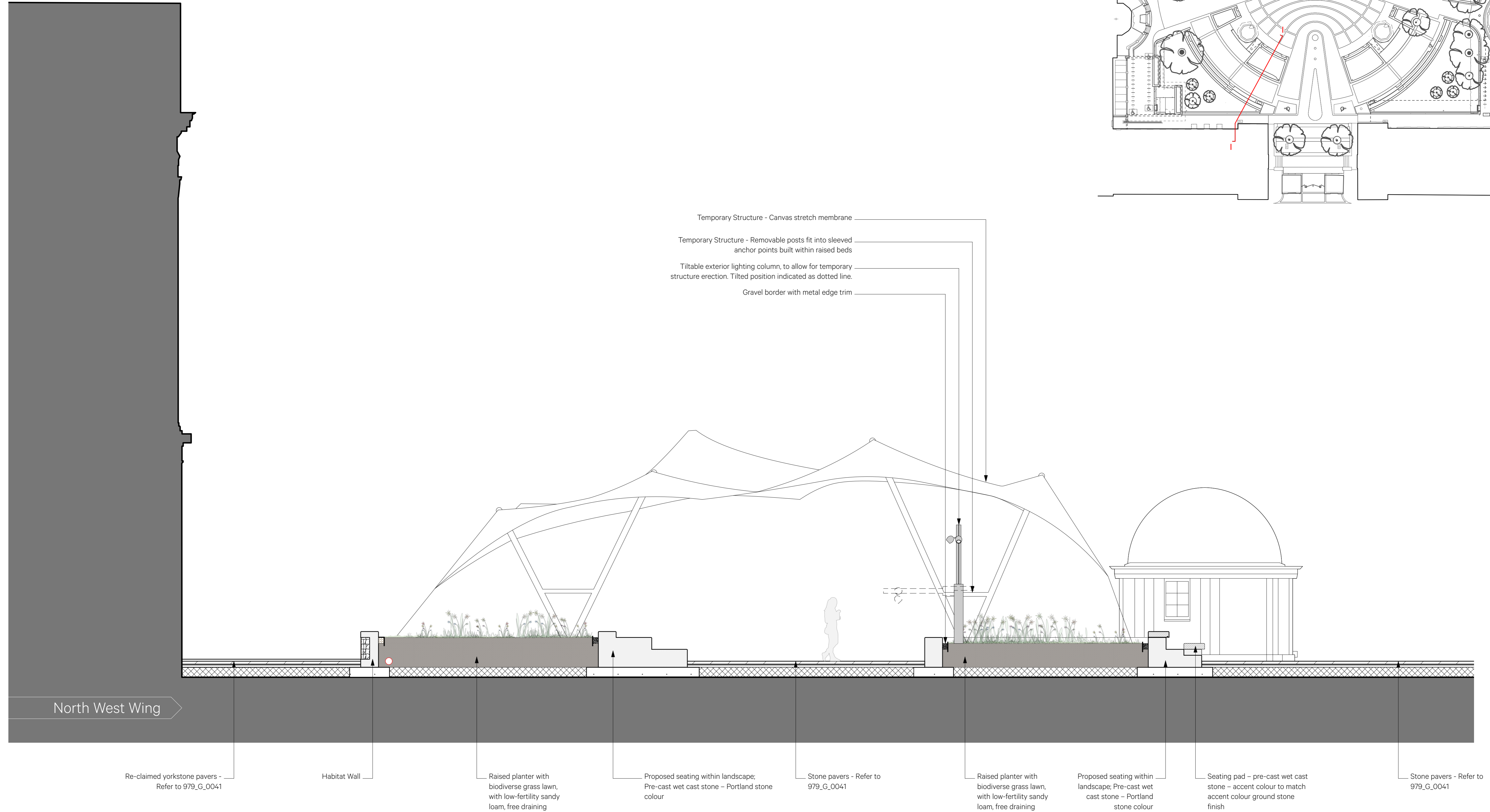
1 Section Through Temporary Structure - Section I - I Scale: 150 @ A1
