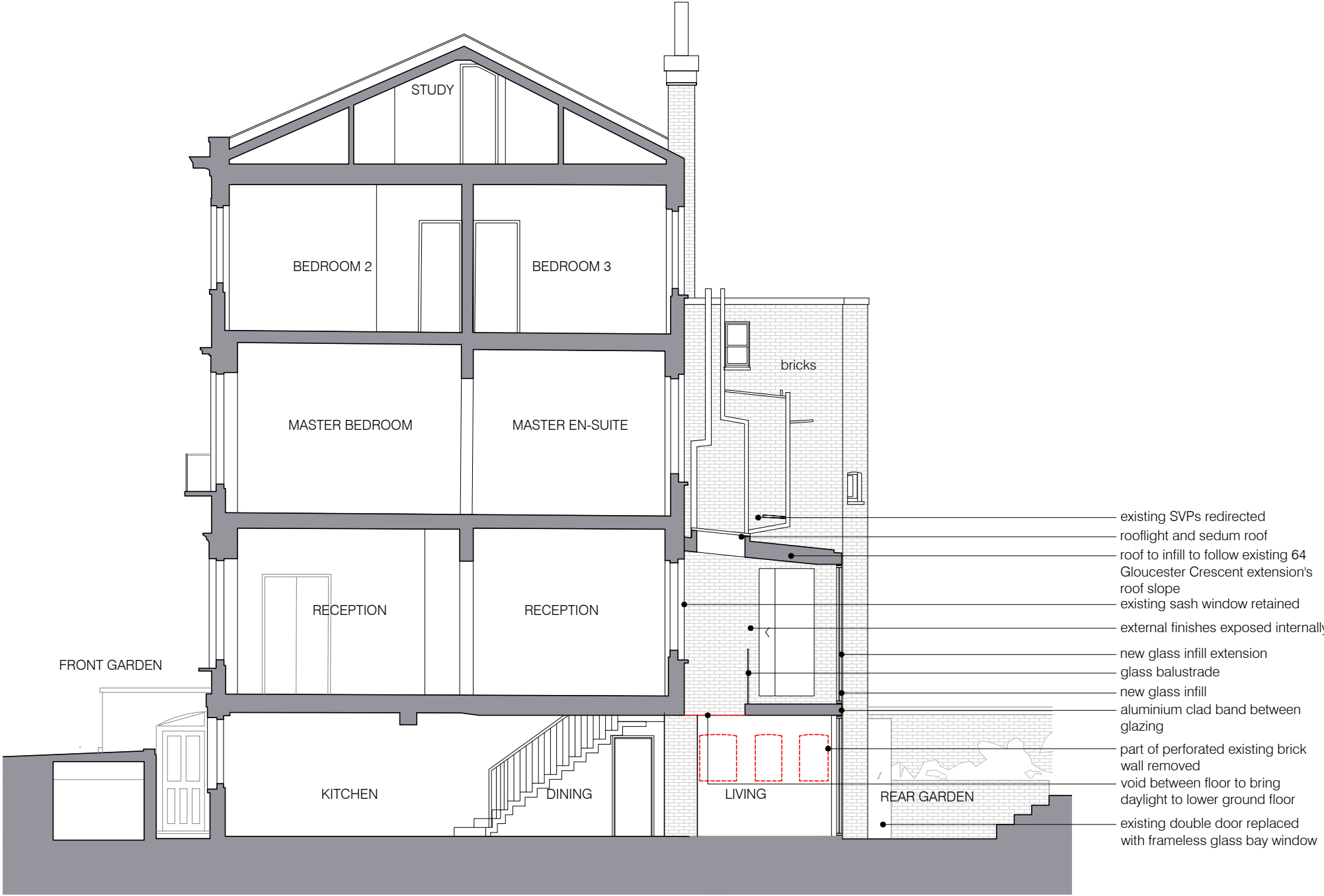
01 PROPOSED SECTION A-A scale 1:100
