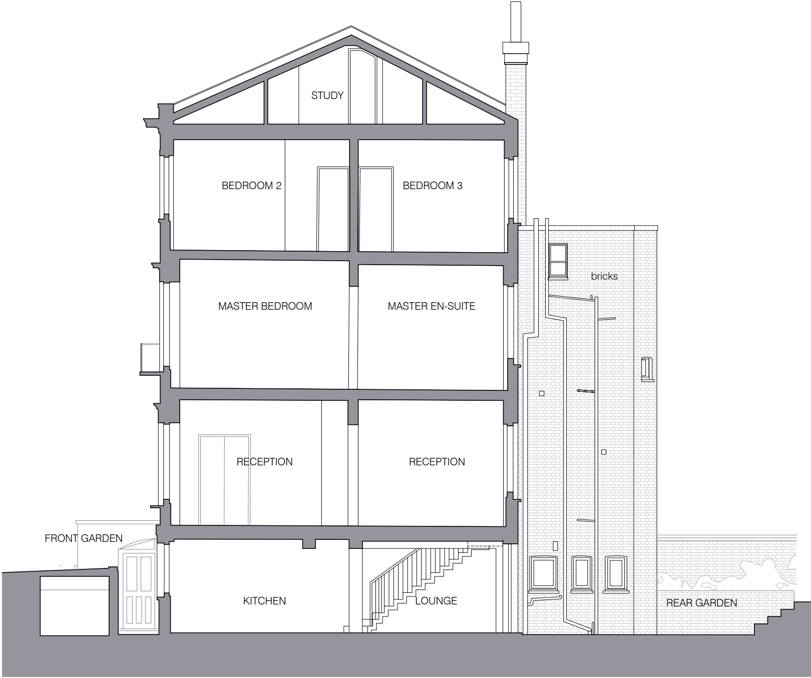
01 EXISTING SECTION A-A scale 1:100
