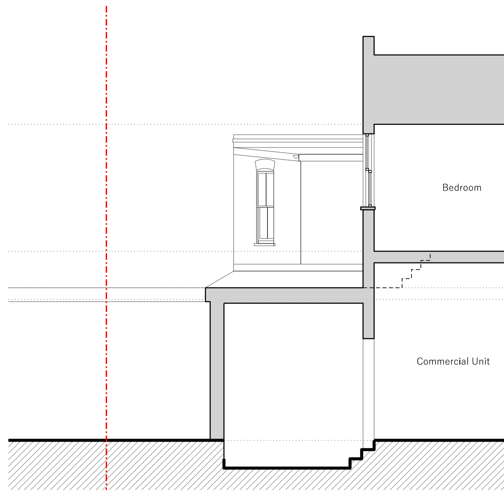
Existing Side Elevation / Section
