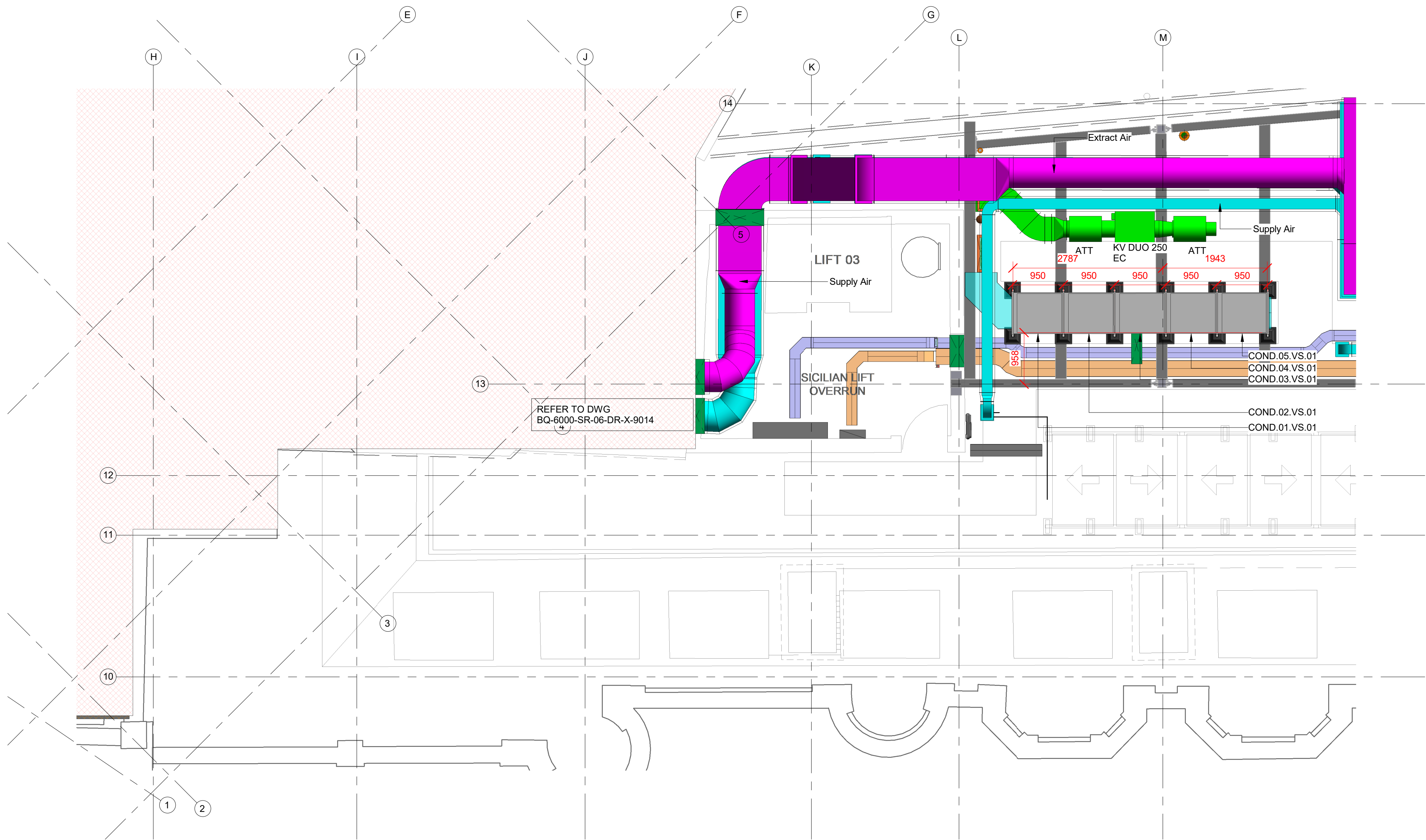
1 Level 06 - SHEET VIEW - COORDINATED SERVICES - VSH SCALE: 1: 50
