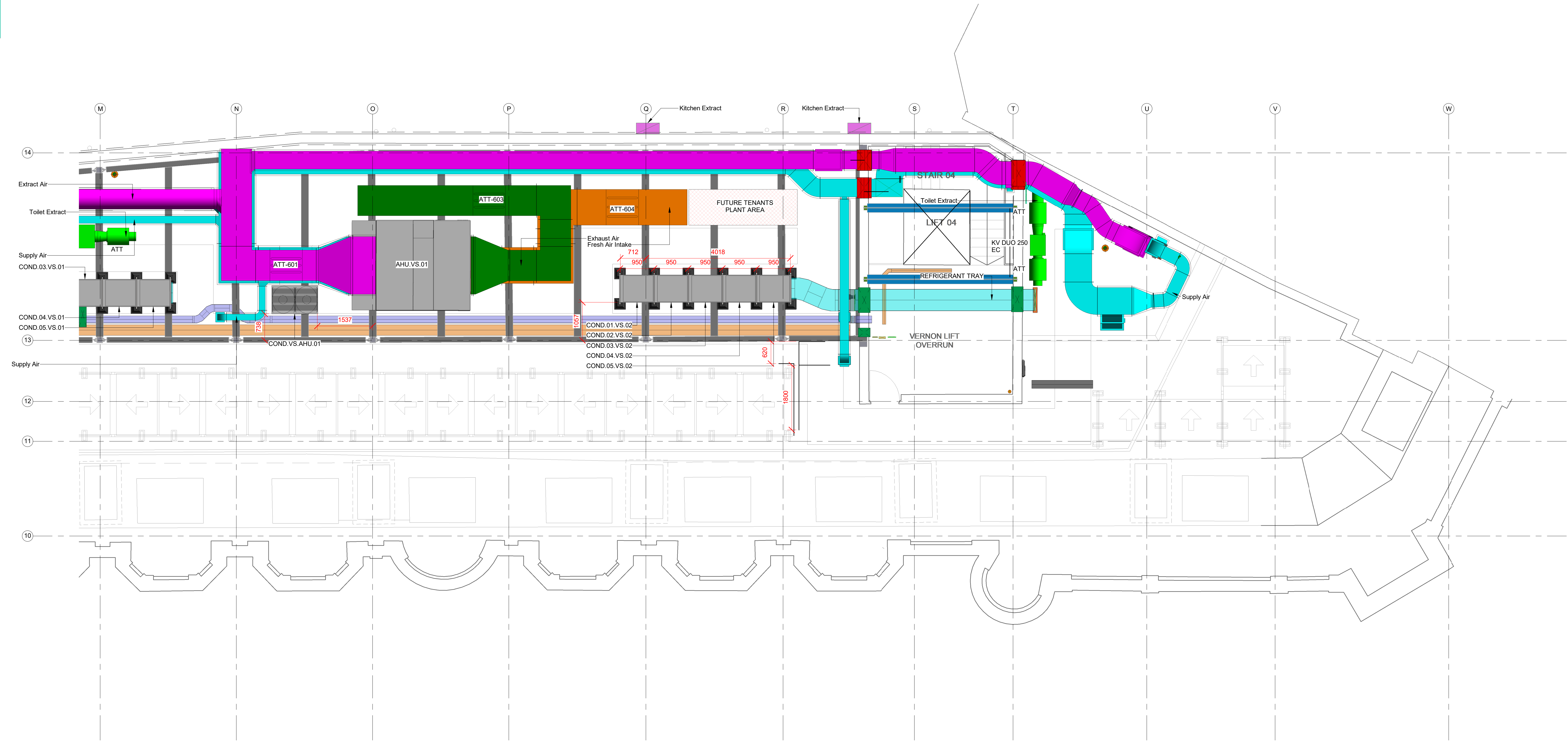
1 Level 06 - SHEET VIEW - COORDINATED SERVICES - VSH SCALE: 1: 50
