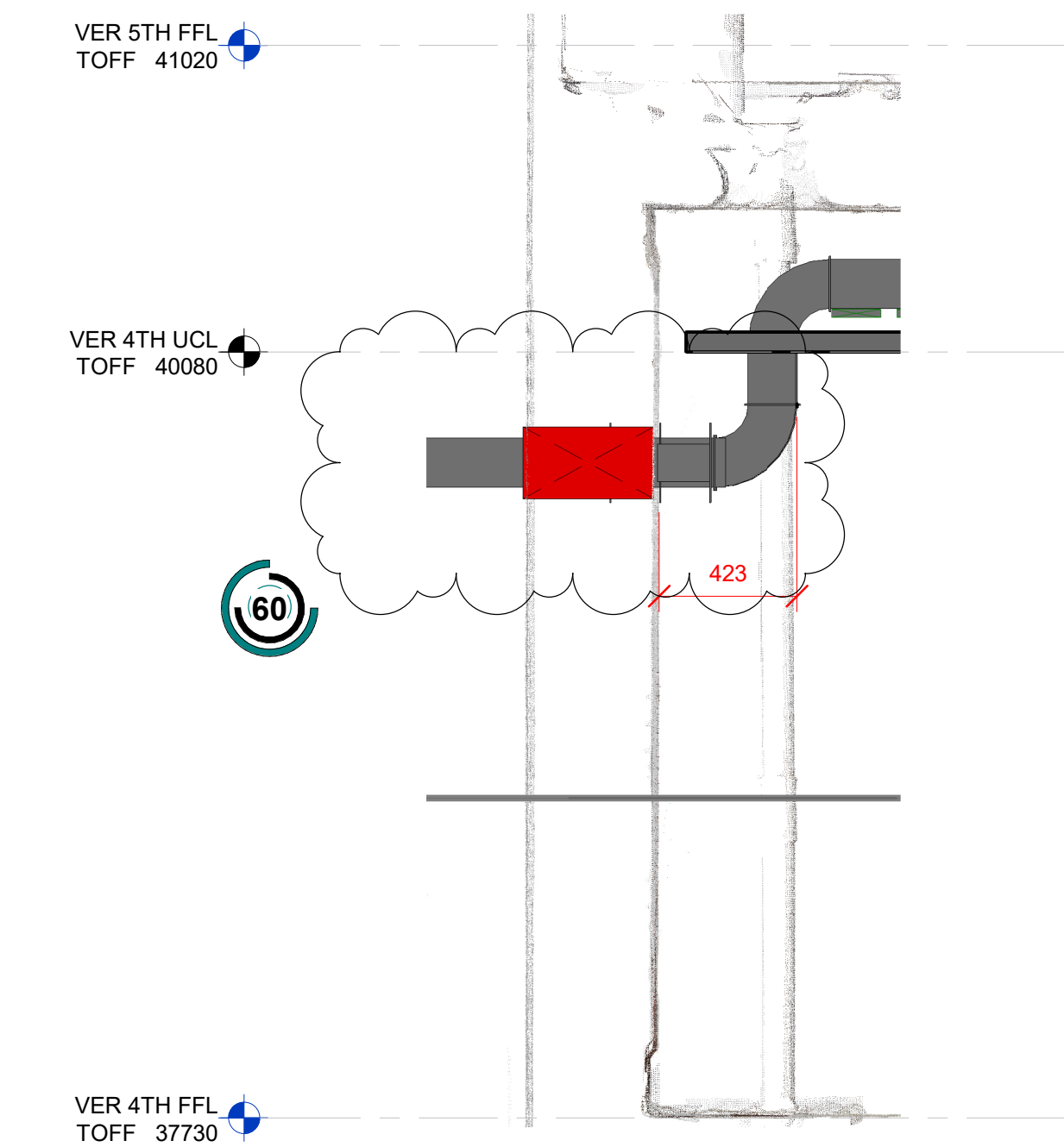
1. Section East Supply - Lightwell SCALE: 1 : 20
