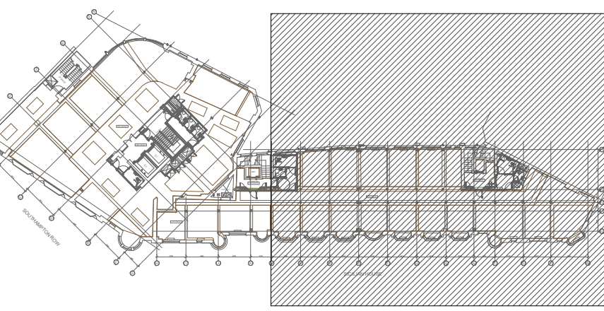
KEYPLAN
