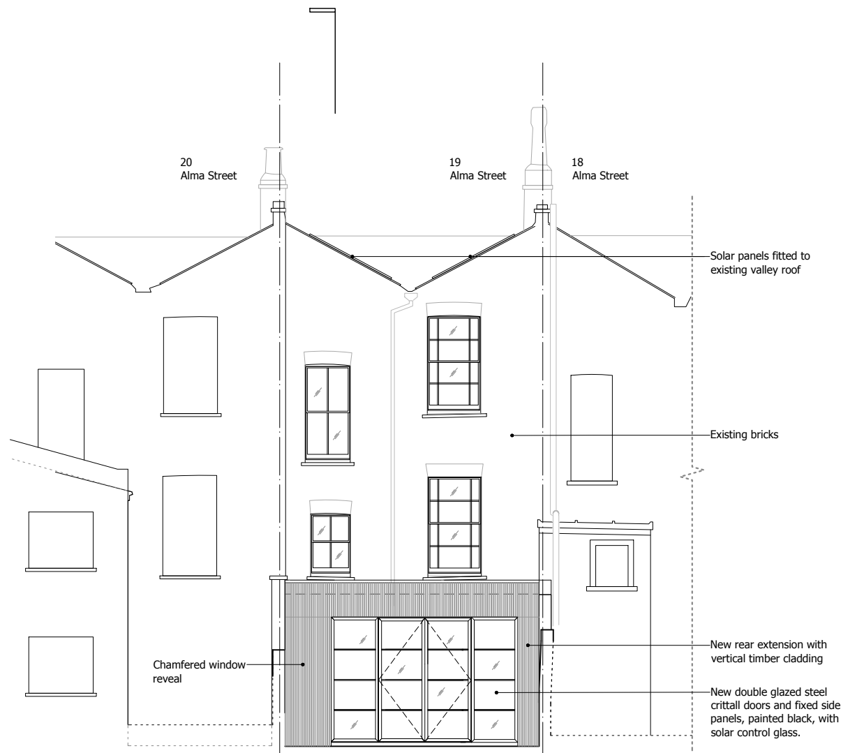
REAR ELEVATION
