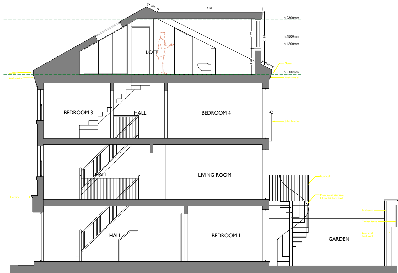
Section A-A as proposed 1:100 @A3
