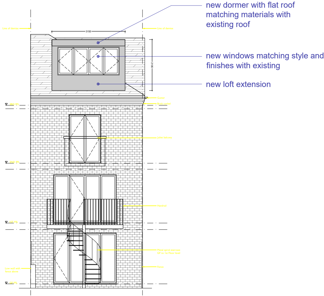
Rear elevation as proposed 1:100 @A3
