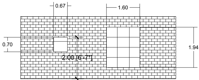
Existing Ground Floor Rear Elevation
