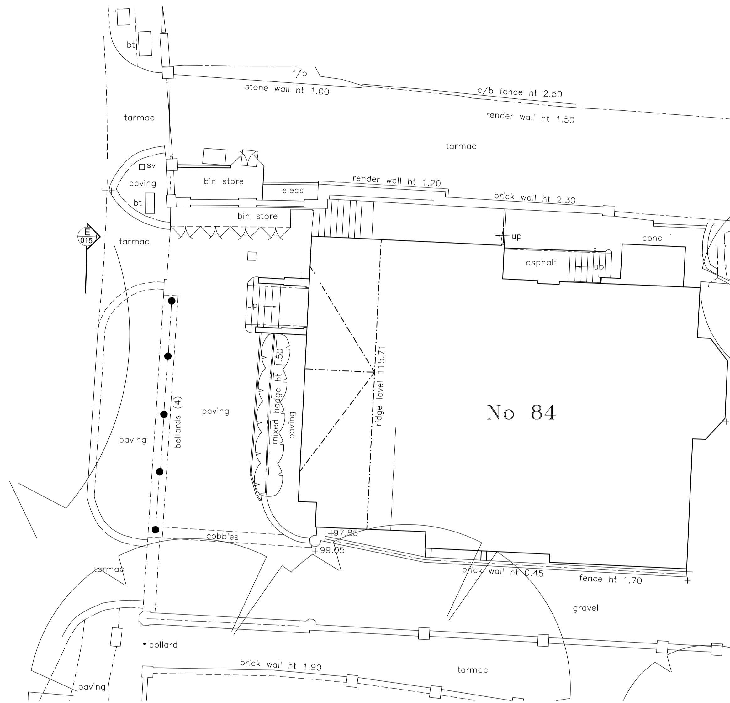
LA-046-015 EXISTING PLAN: NO. 84 FITZJOHN'S AVENUE 01 1:100@A1
