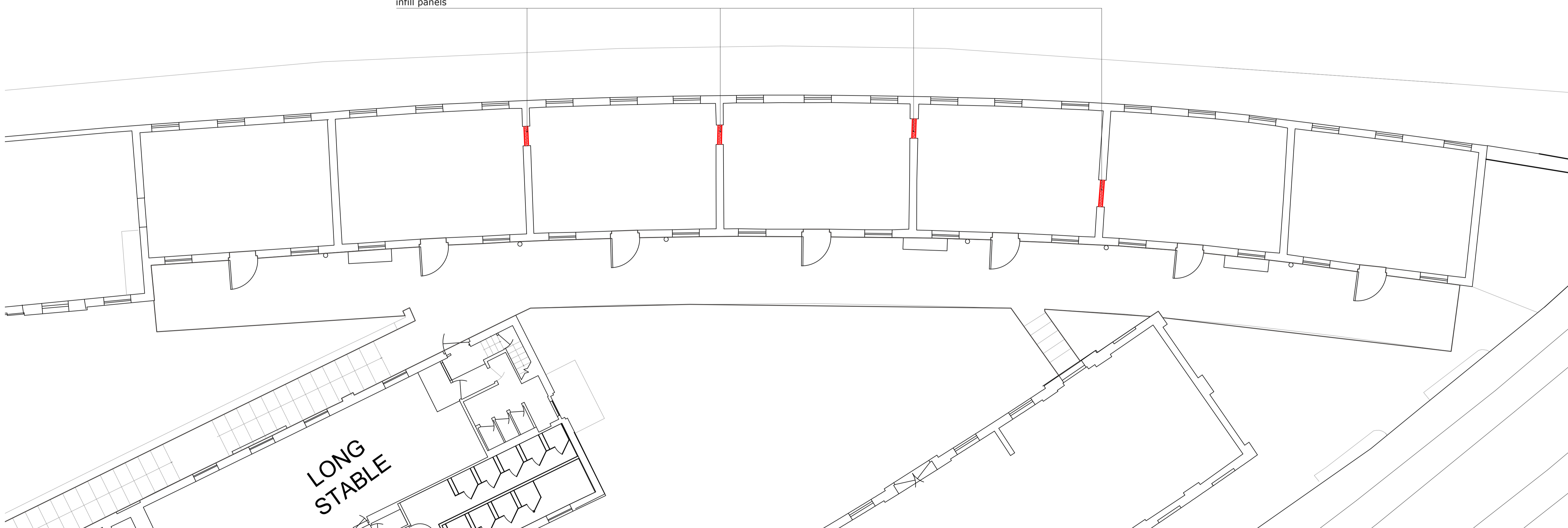
PL FIRST FLOOR DEMOLITION PLAN 1:100@A1, 1:200@A3
