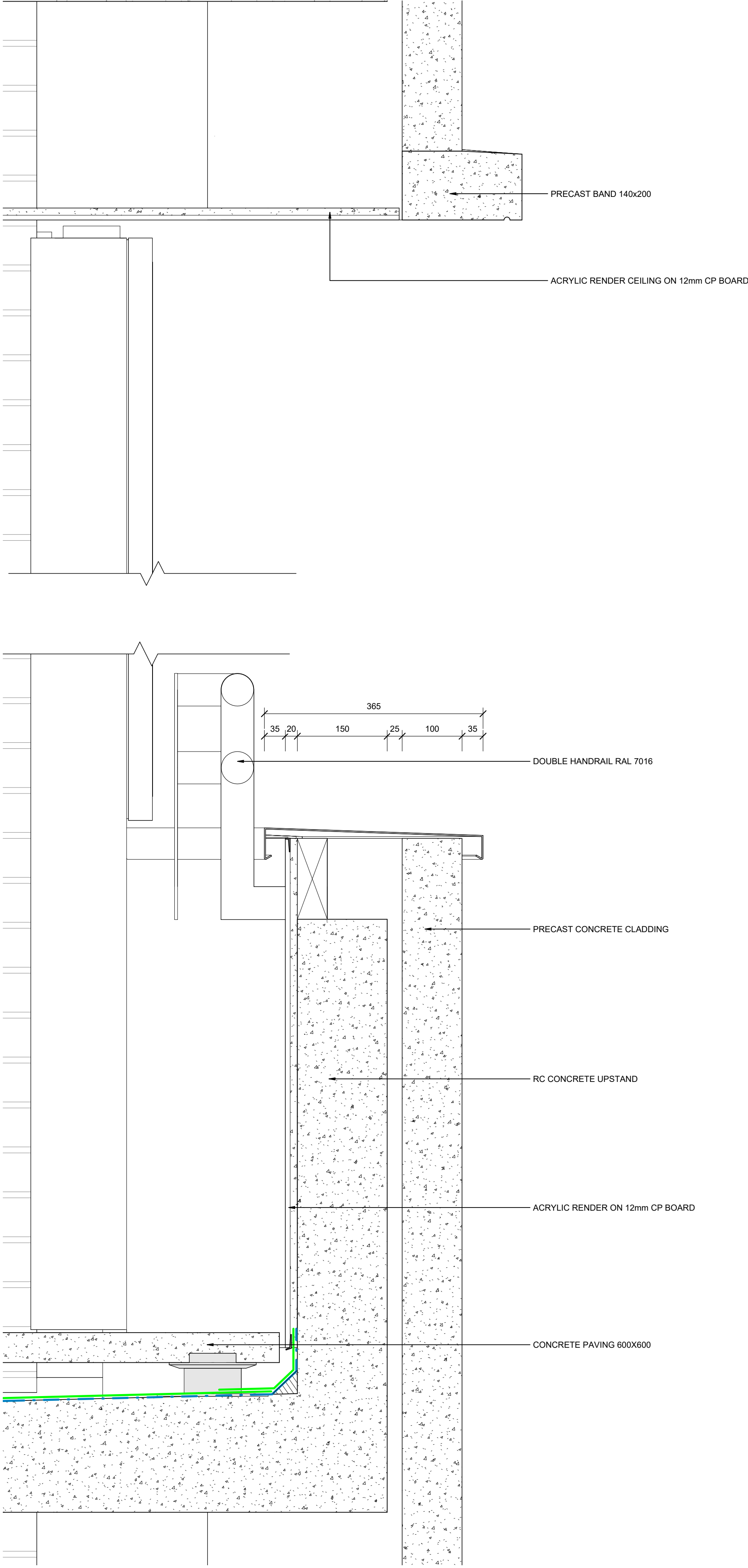
pl.06 Inset Balcony - Detail 1 : 5
