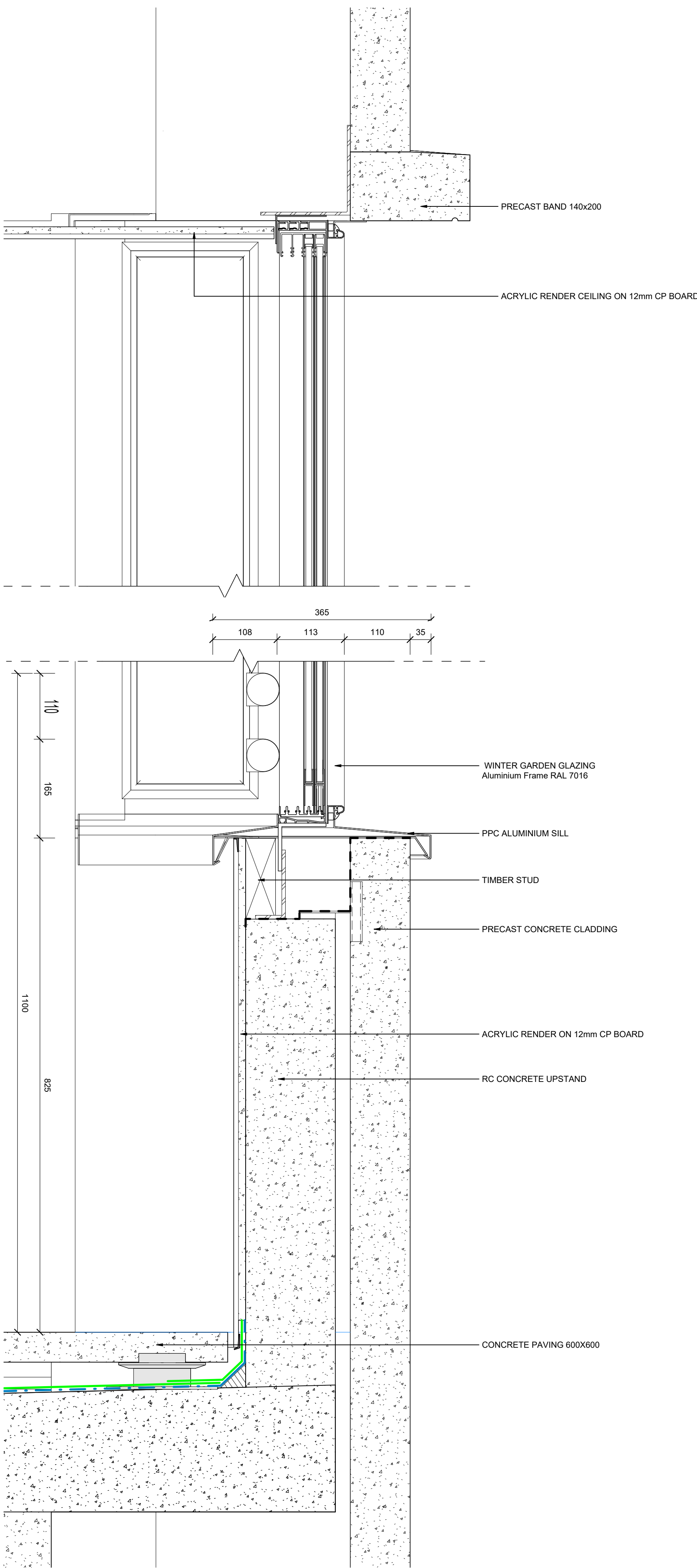
pl.05 Winter Garden Glazing - Sill and Head Detail 1 : 5
