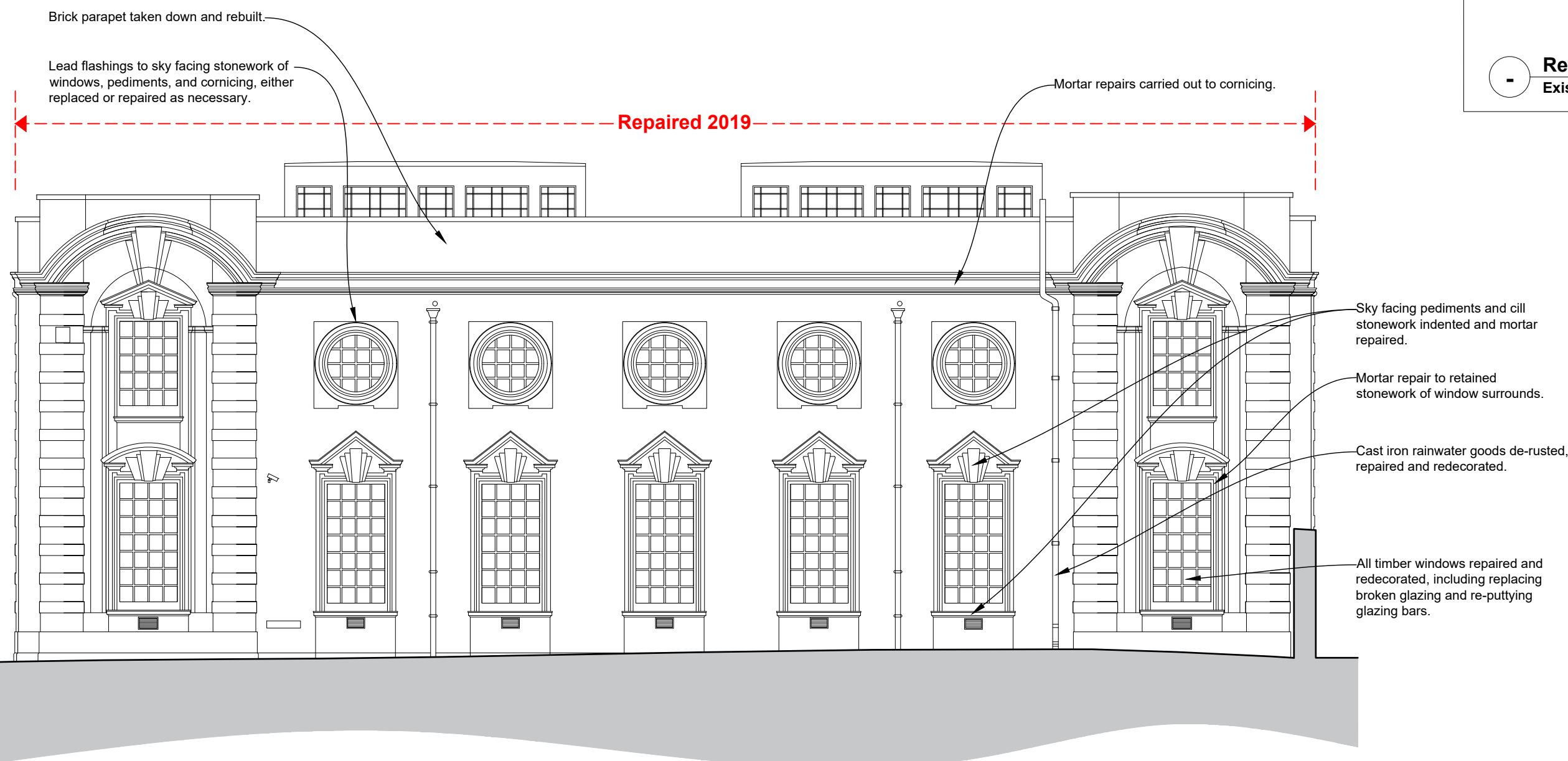
1 East Elevation Existing
