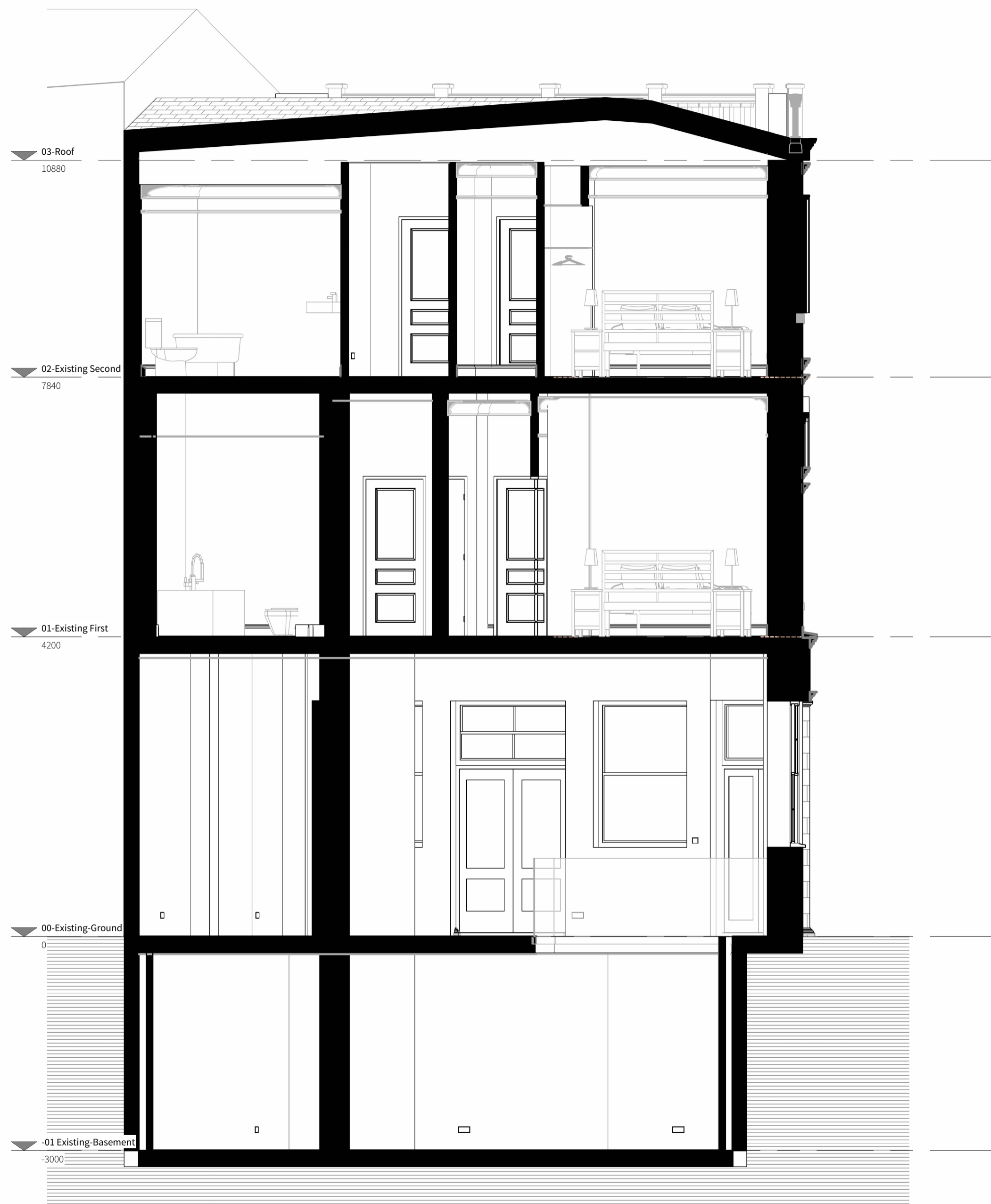
1 PROPOSED - Section B 1:50
