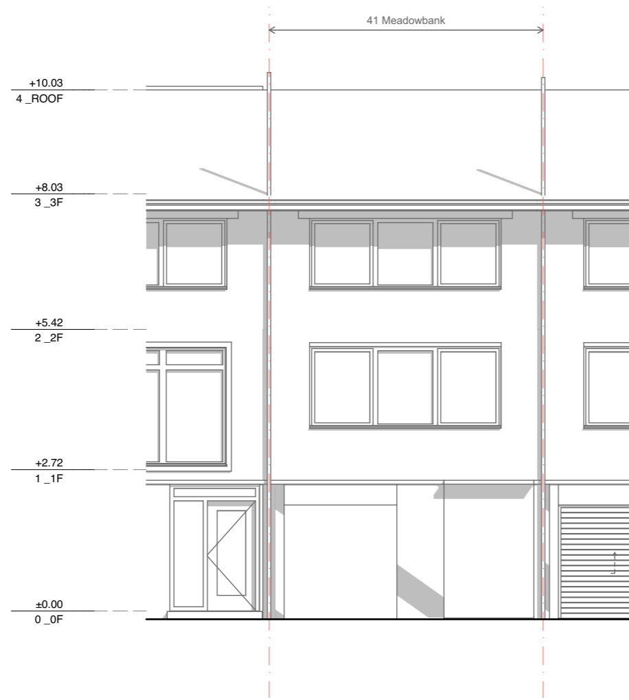
FRONT ELEVATION
