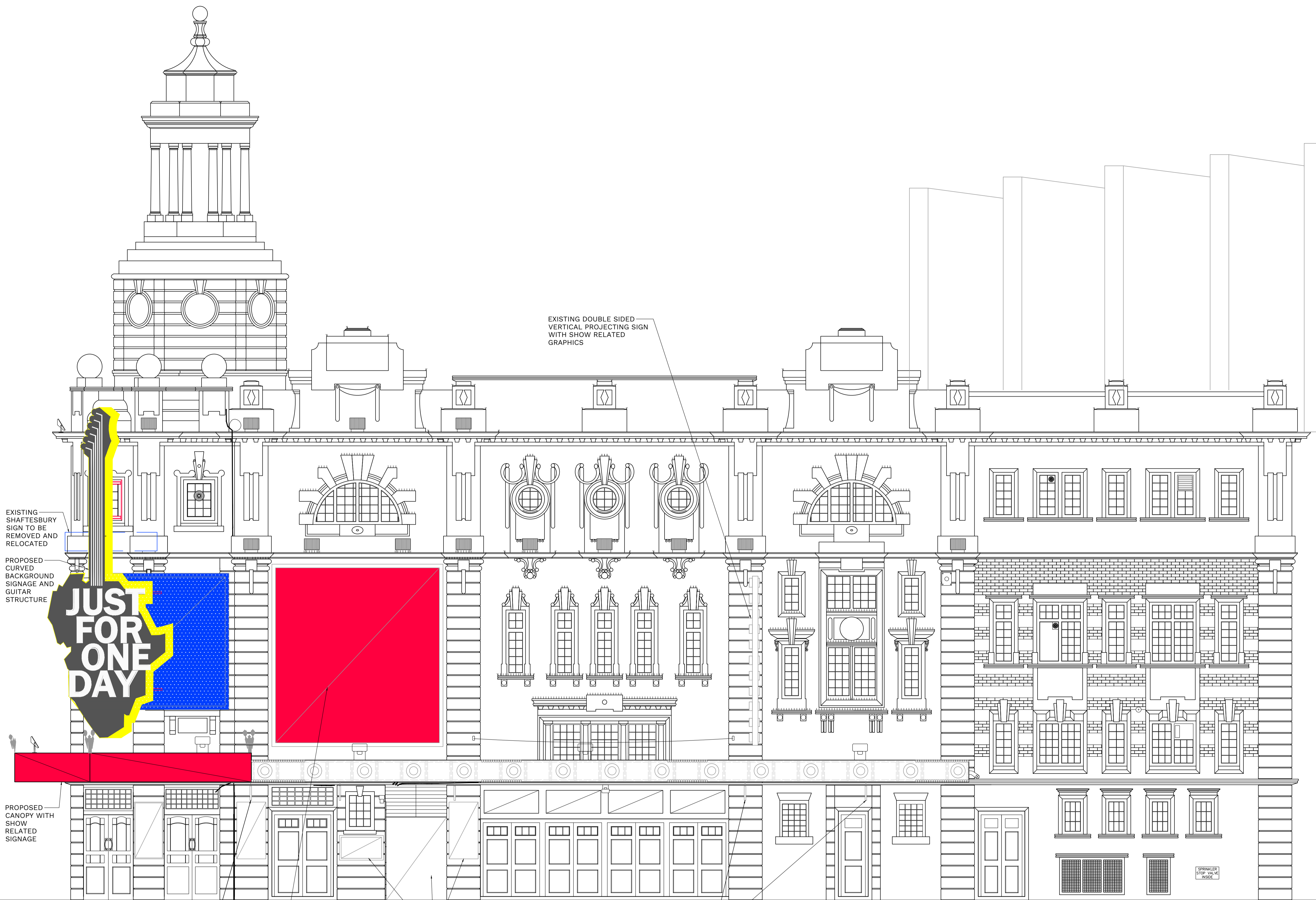
PROPOSED ELEVATION ON HIGH HOLBORN (SCALE 1:50 AT A1)
