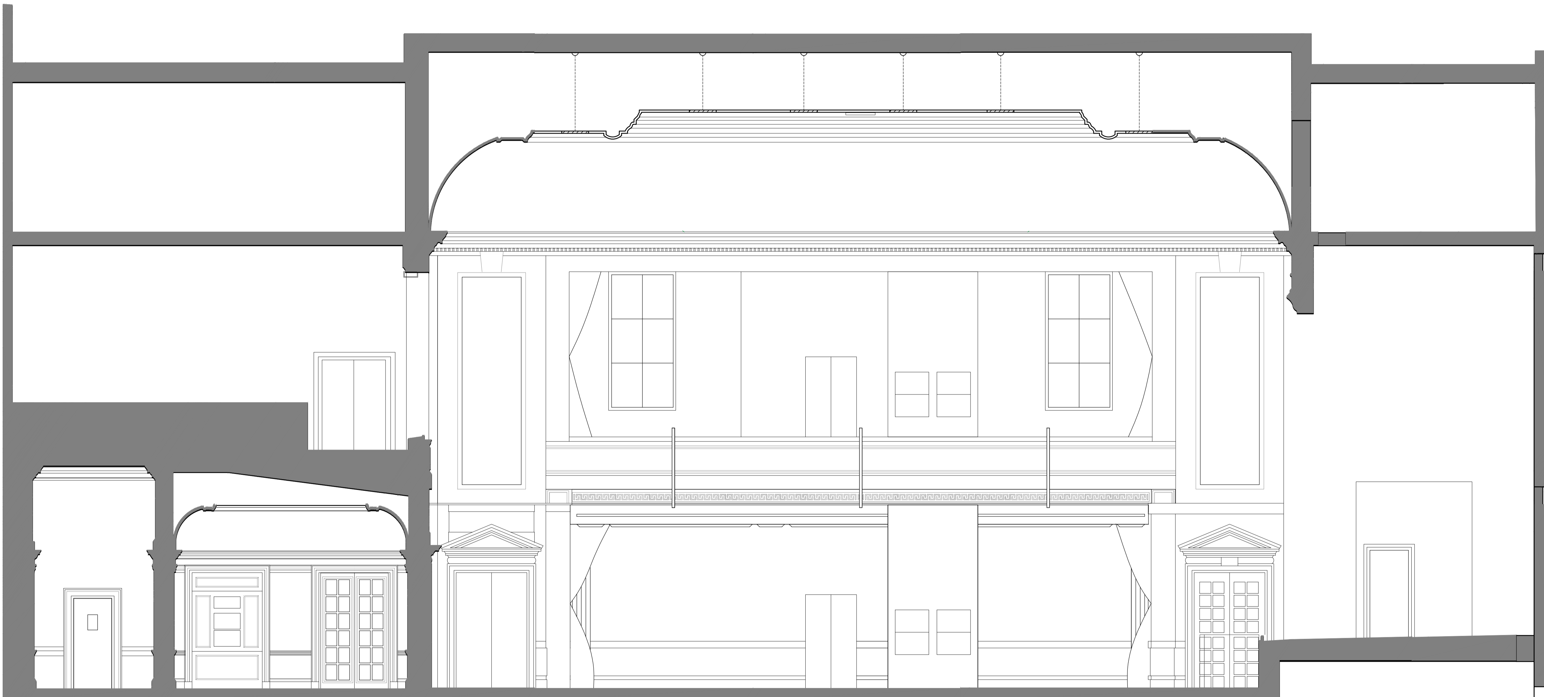
1 EXISTING INTERNAL ELEVATION - WEST 0015 1:50 @ A1
