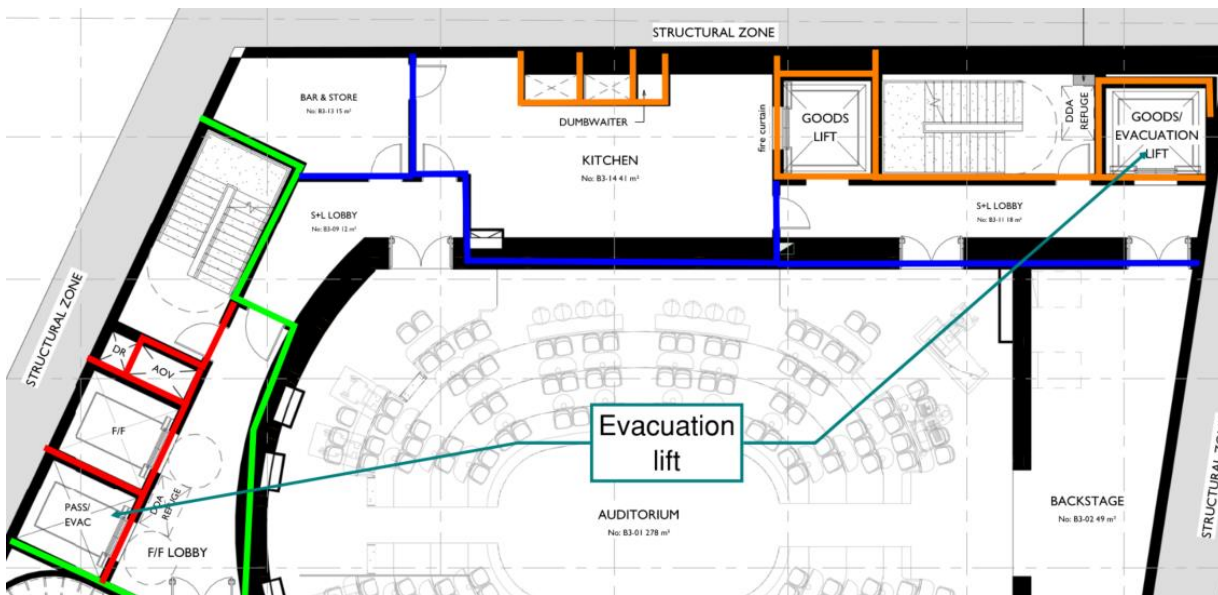
Figure 7: Location of Evacuation Lifts in theatre portion of the building
