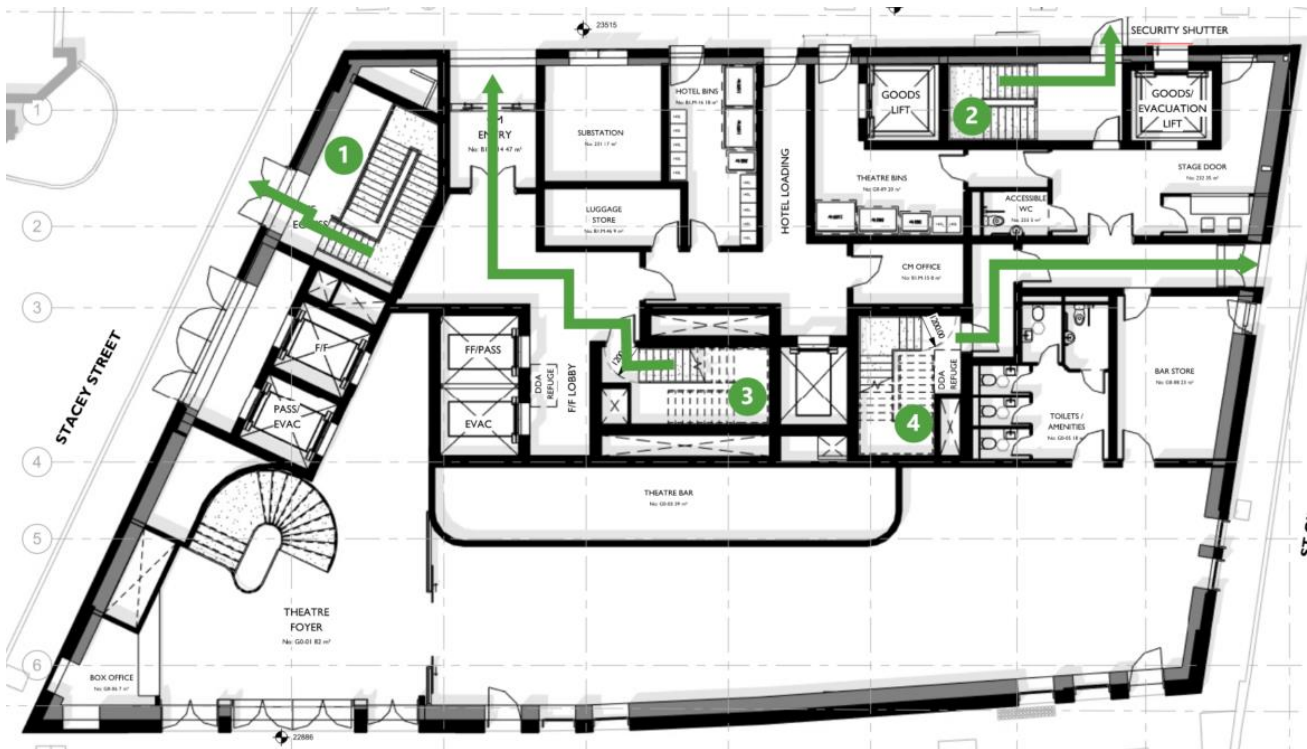
Figure 6 Final Exits at Ground Floor
