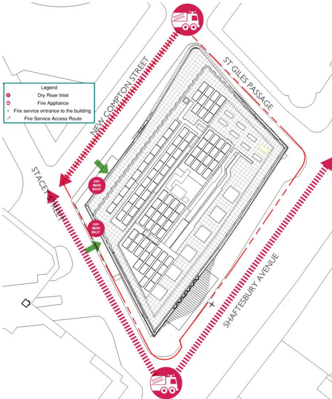
Figure 9 Firefighting access
