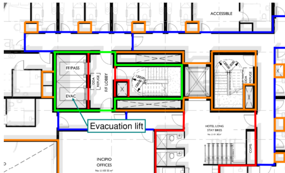
Figure 8: Location of Evacuation Lift in hotel portion of the building
