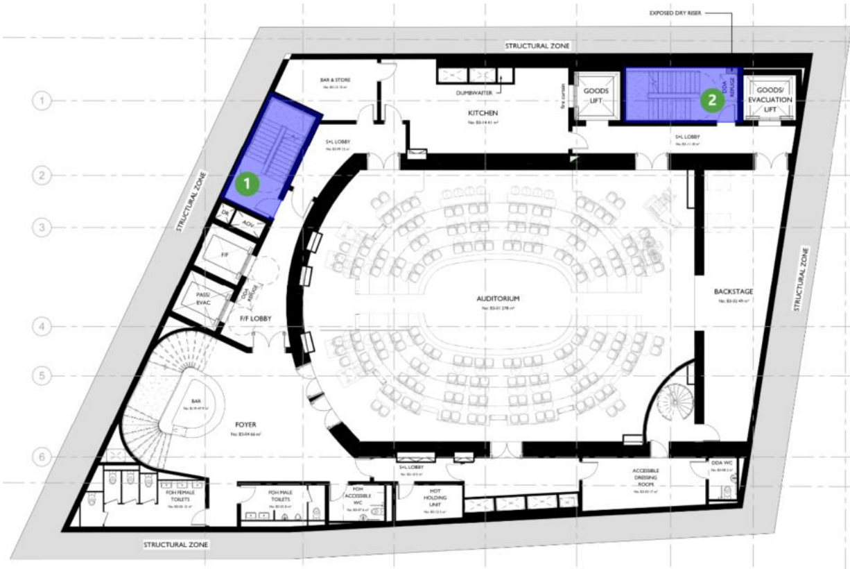
Figure 4: Theatre stair locations on a typical floor and assigned numbers. (The internal layout is only a representation and subject to change)
