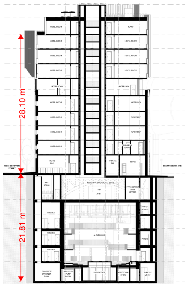
Figure 3 Long section through the Saville Theatre redevelopment showing the height from fire service access level (ground) to the top occupied storey and depth of Basement 4.
