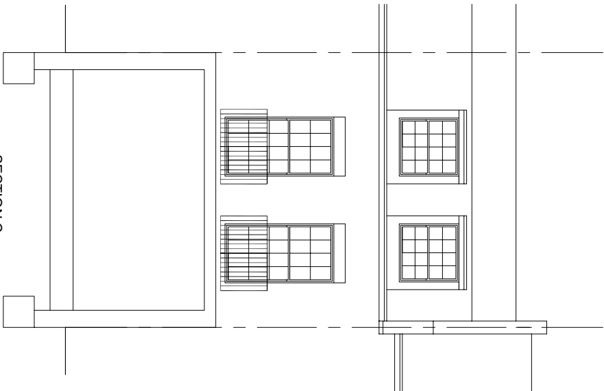
SECTION C
