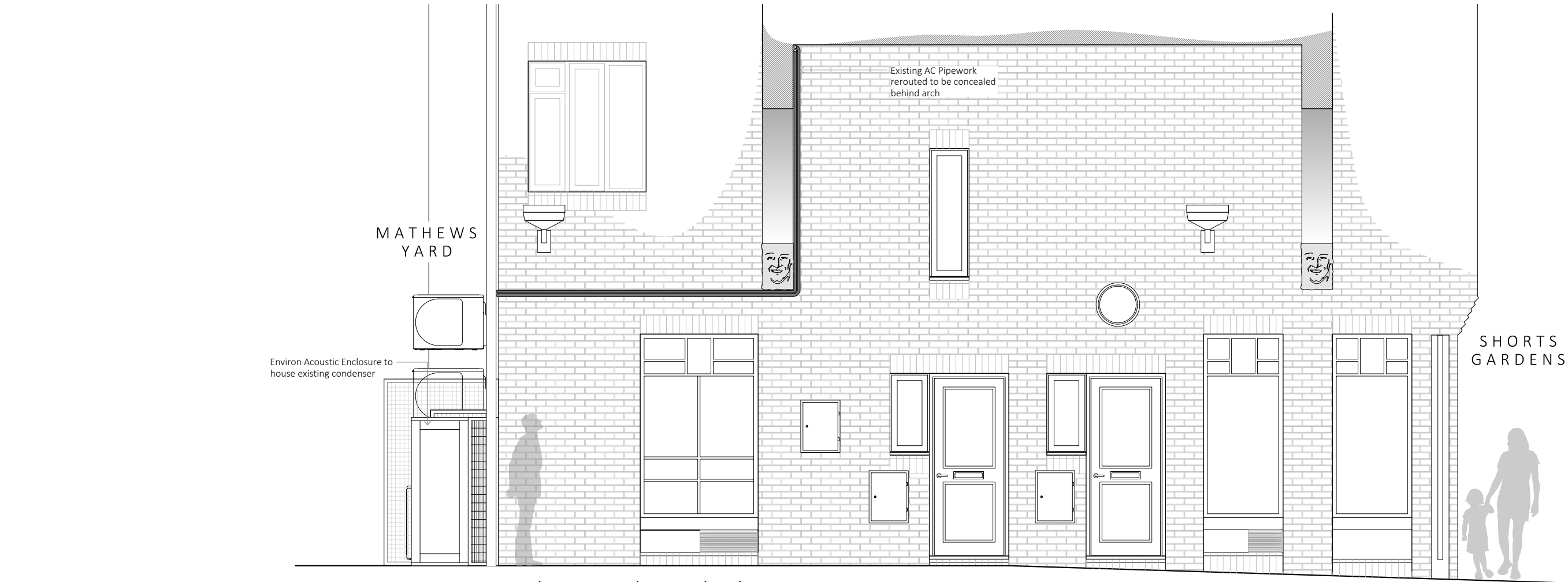
29 Shorts Gardens Side Elevation
