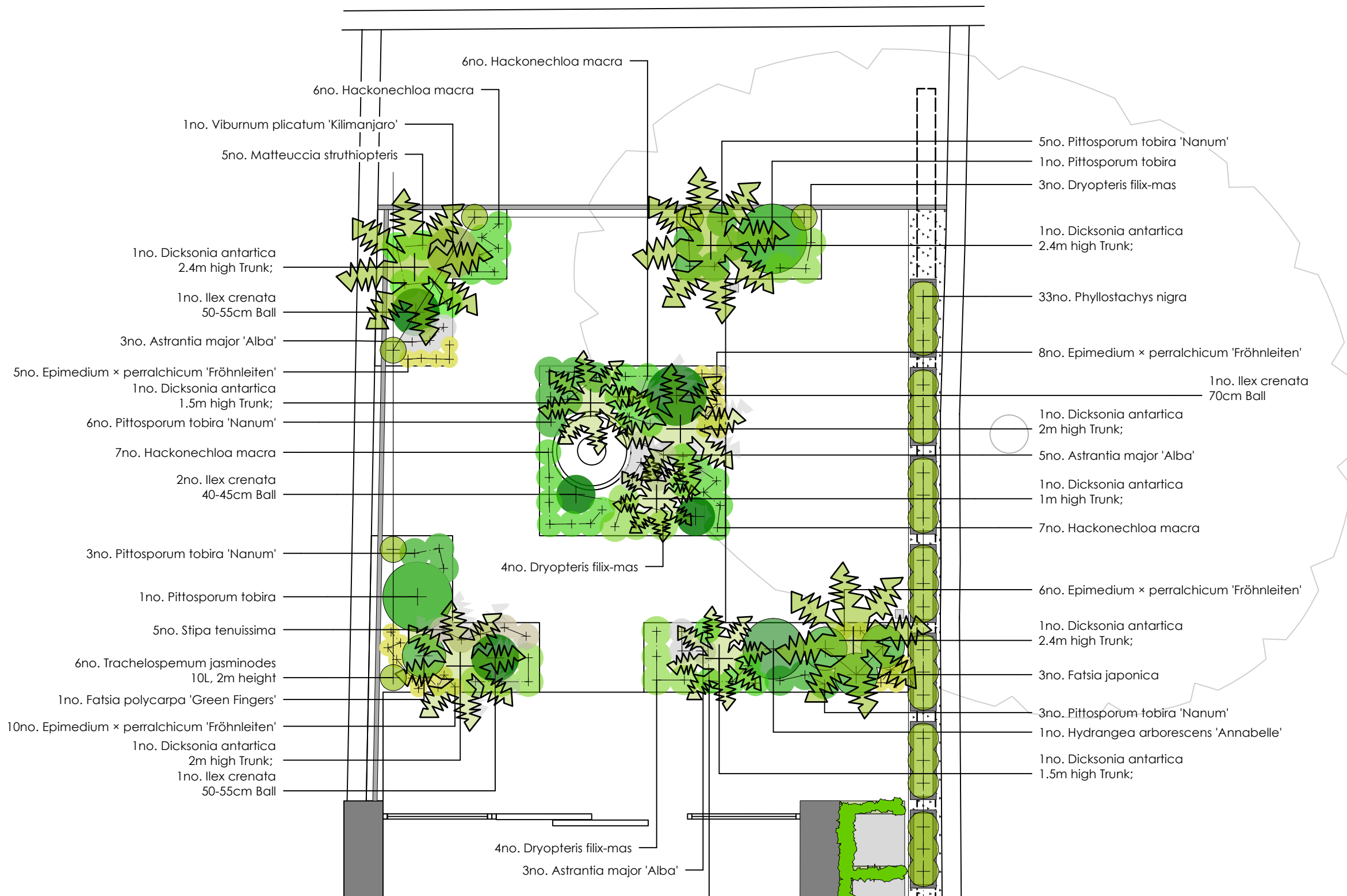
1 REAR GARDEN PLANTING SETTING OUT PLAN 1:50@A3
