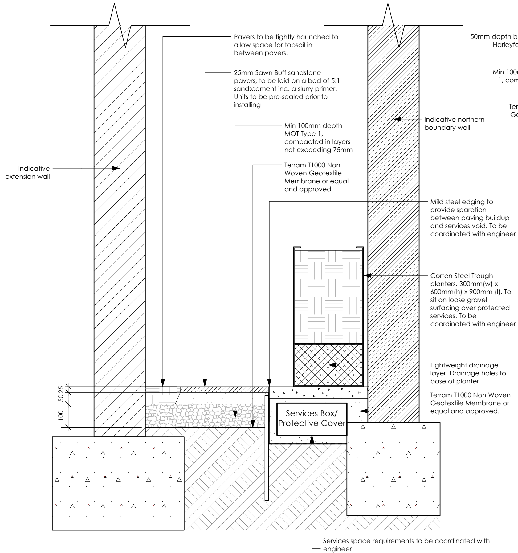
1 SECTION THROUGH PATHWAY NORTH OF PROPOSED EXTENSION 1:10@A3
