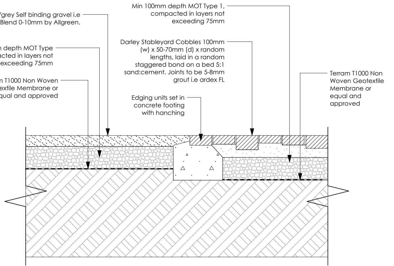
2 SANDSTONE COBBLES AND SELF BINDING GRAVEL INTERFACE SECTION 1:10@A3
