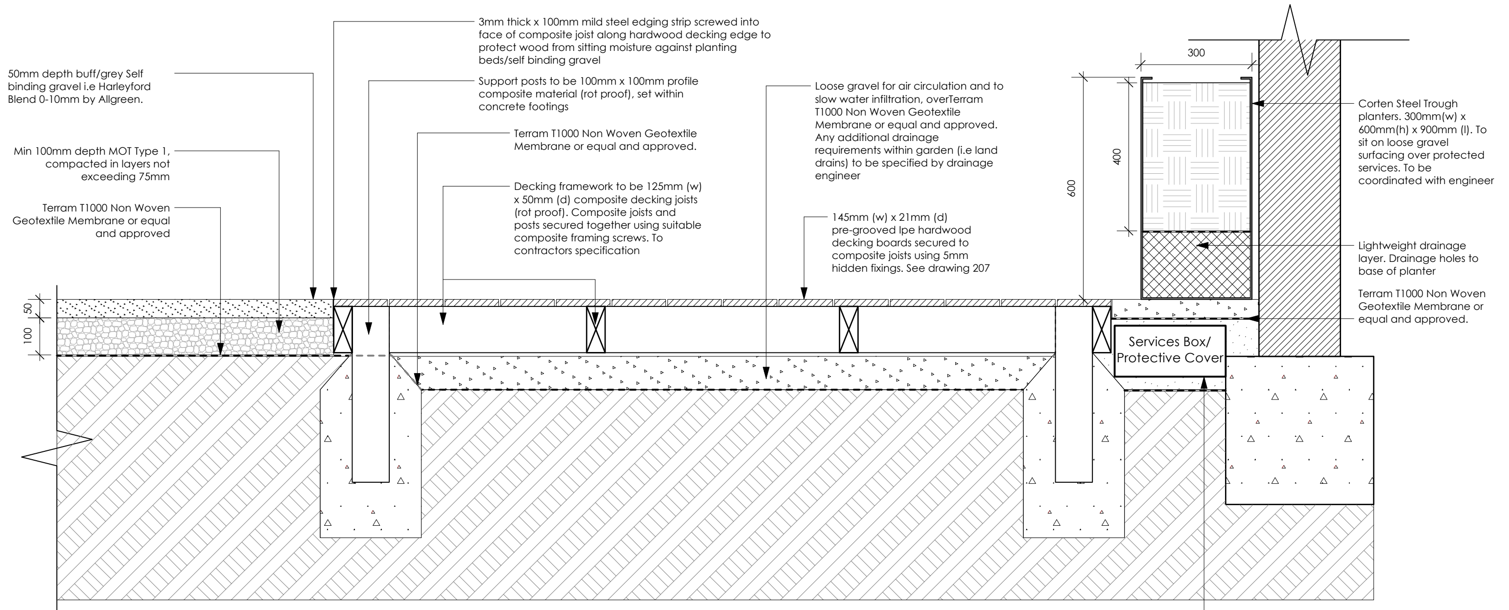
1 SECTION THROUGH SELF BINDING GRAVEL, DECKING AND NORTHERN BOUNDARY WALL 1:10@A3
