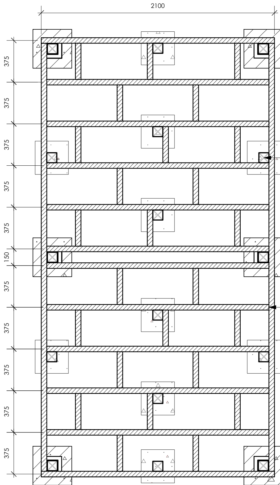
1 INDICATIVE POSTS AND DECKING FRAMEWORK PLAN VIEW 1:20@A3
