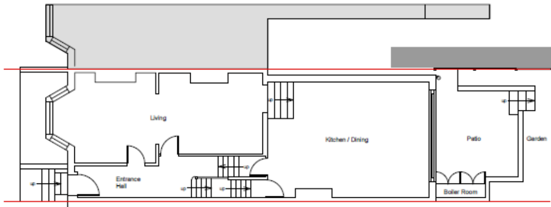
Ground Floor Plan as Existing - 1:100 Ⓞ
