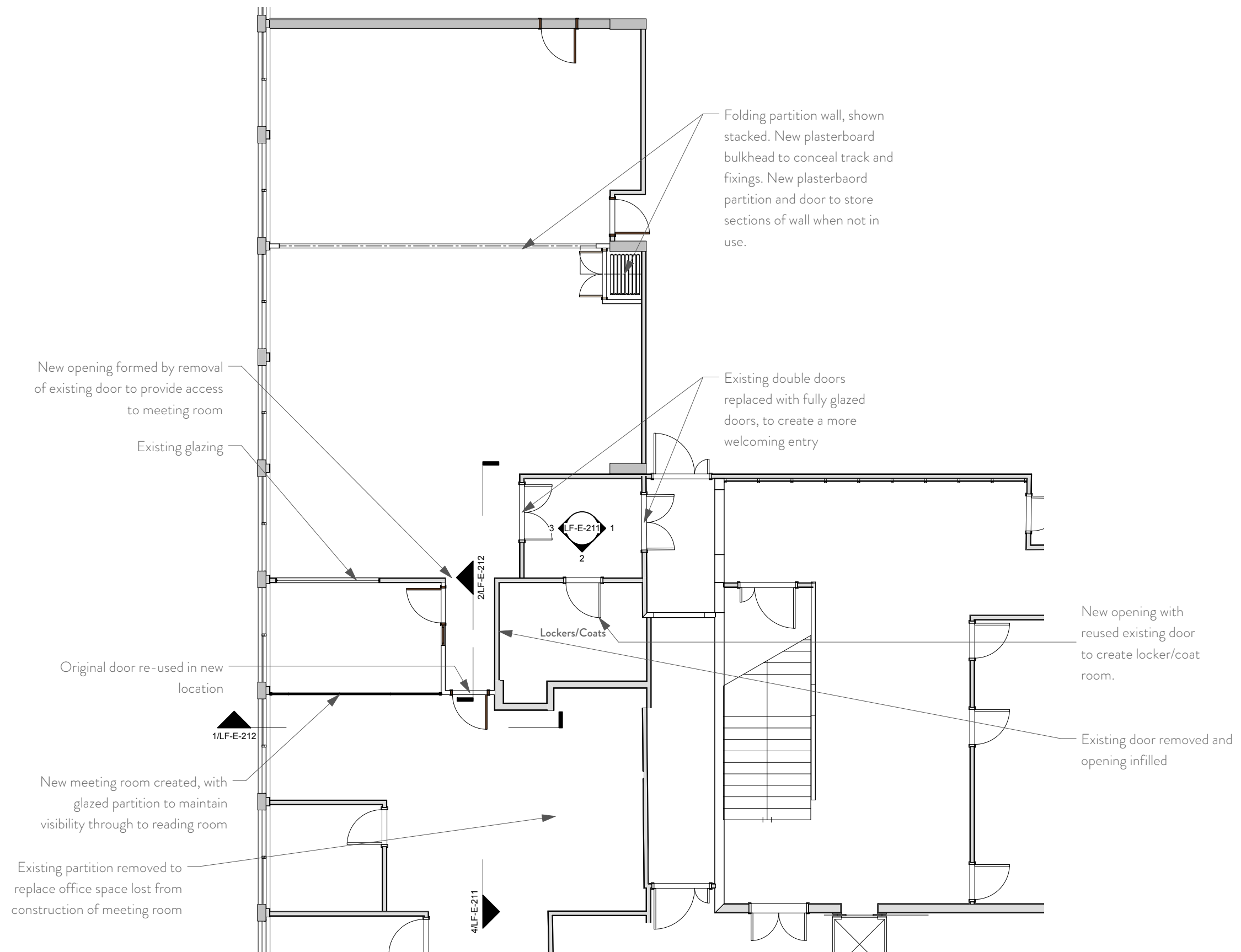
1 Level F Special Collections Reading Room Plan Scale: 1:100
