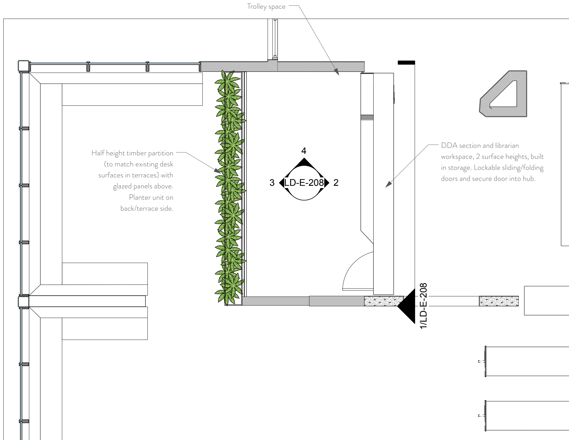
1 Proposed Librarian Hub Level D Scale: 1:50
