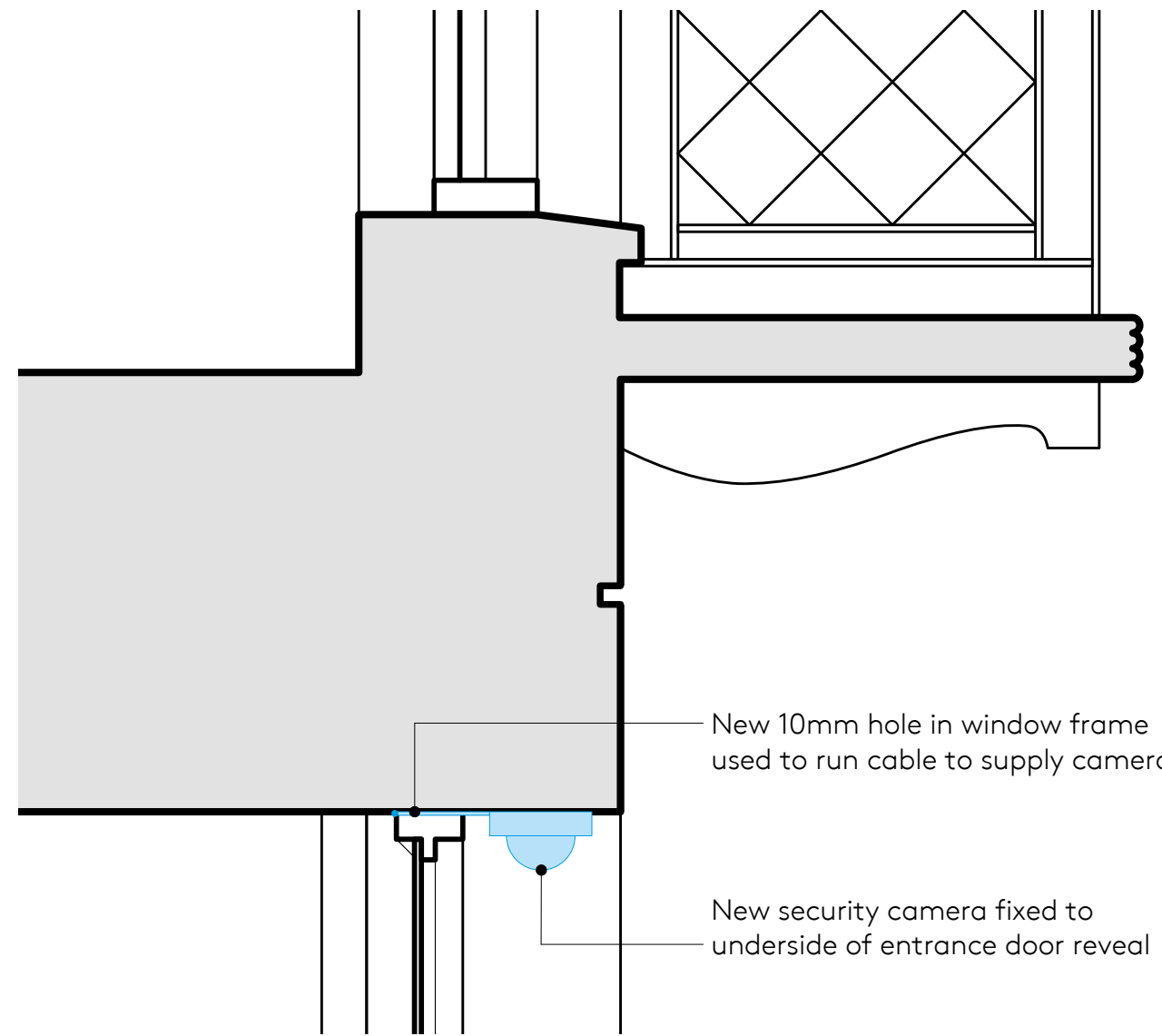
Proposed Section AA Scale: 1:10
