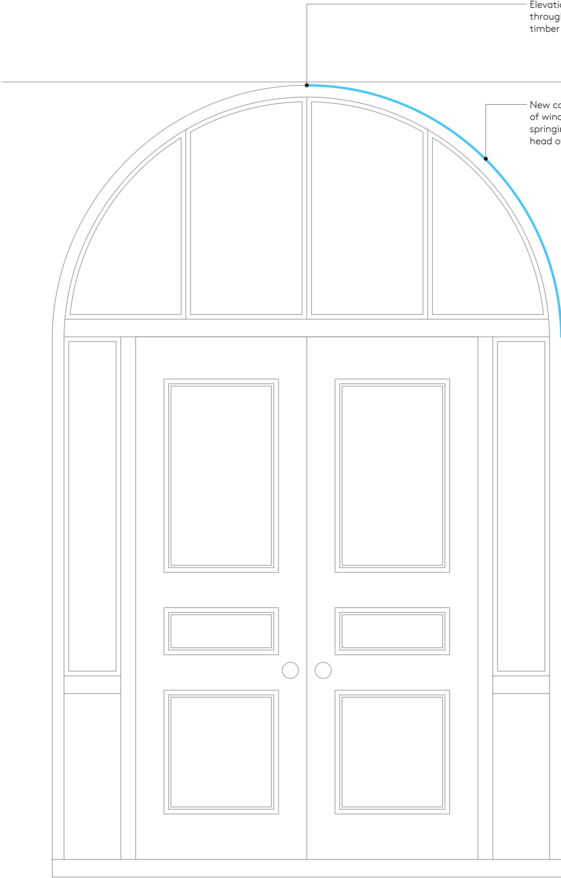
Proposed Internal Elevation Scale: 1:10
