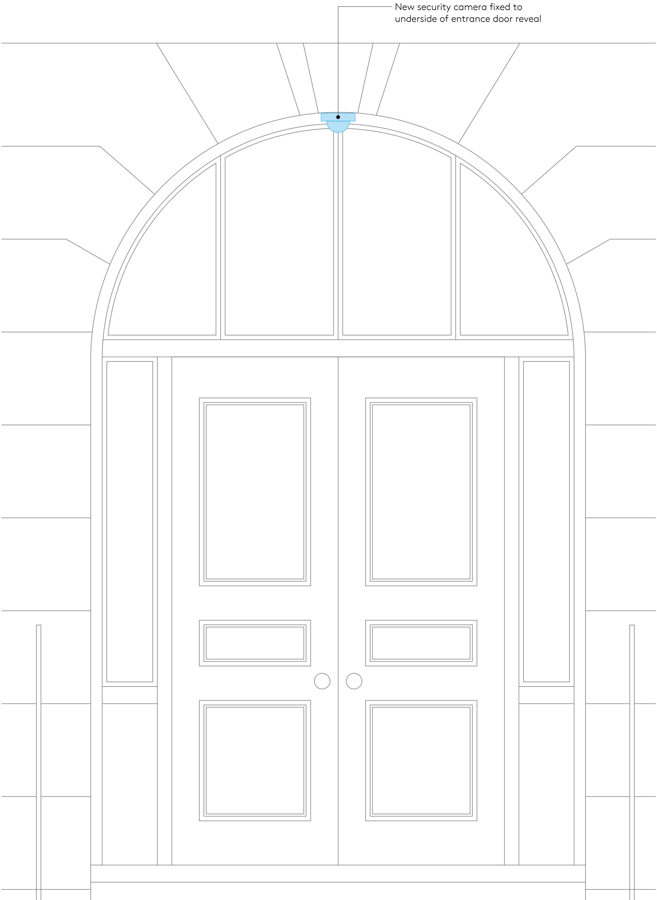
Proposed External Elevation Scale: 1:10
