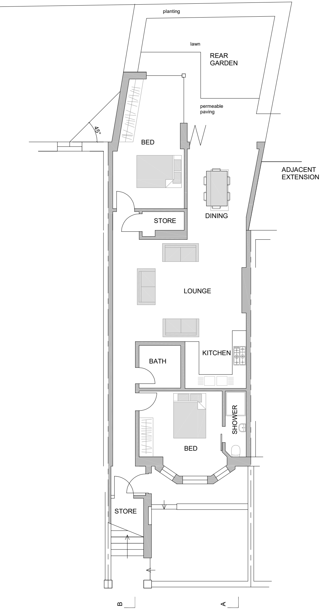
LOWER GROUND FLOOR PLAN 91 M2
