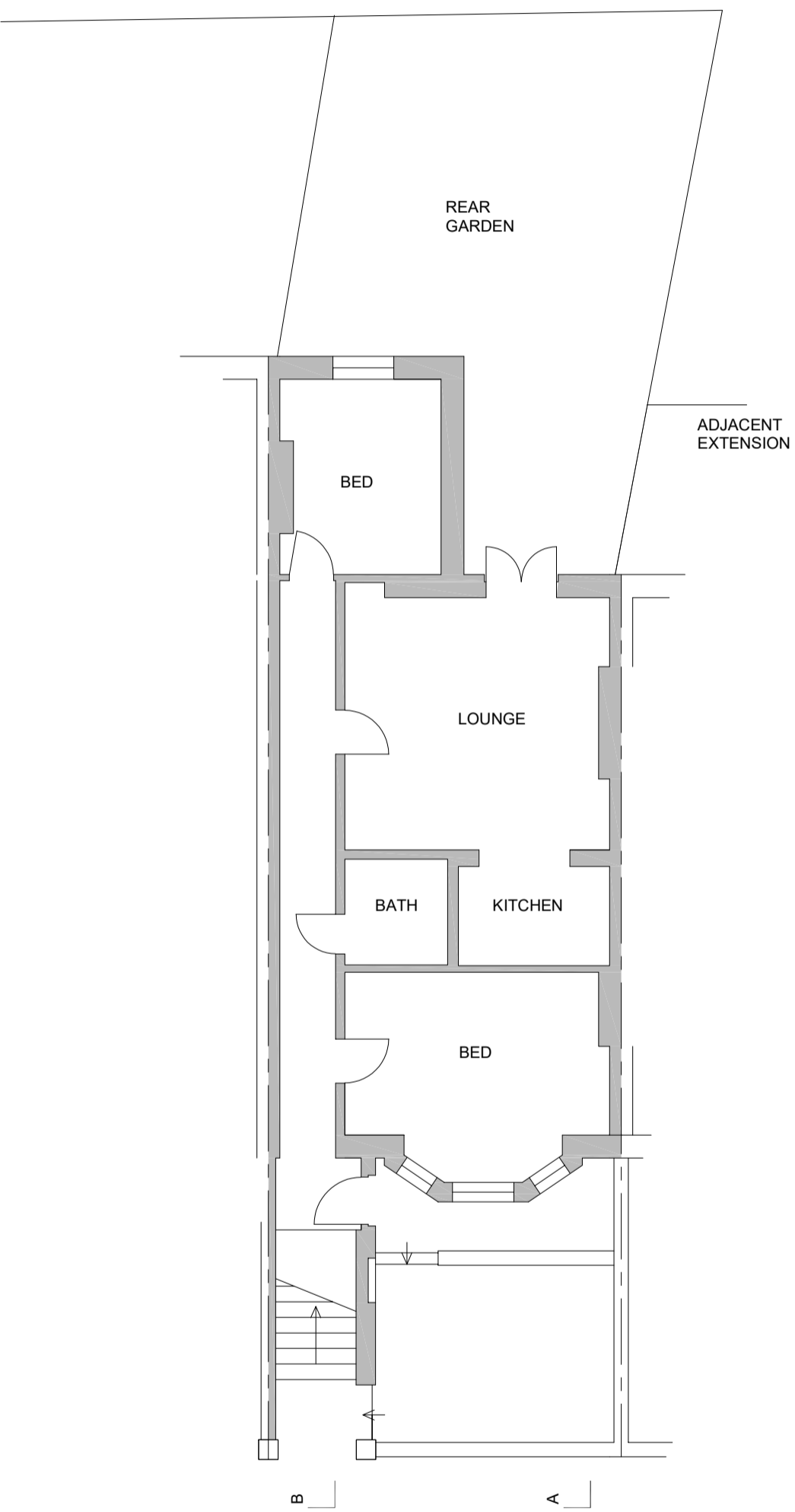
LOWER GROUND FLOOR PLAN 68 M2
