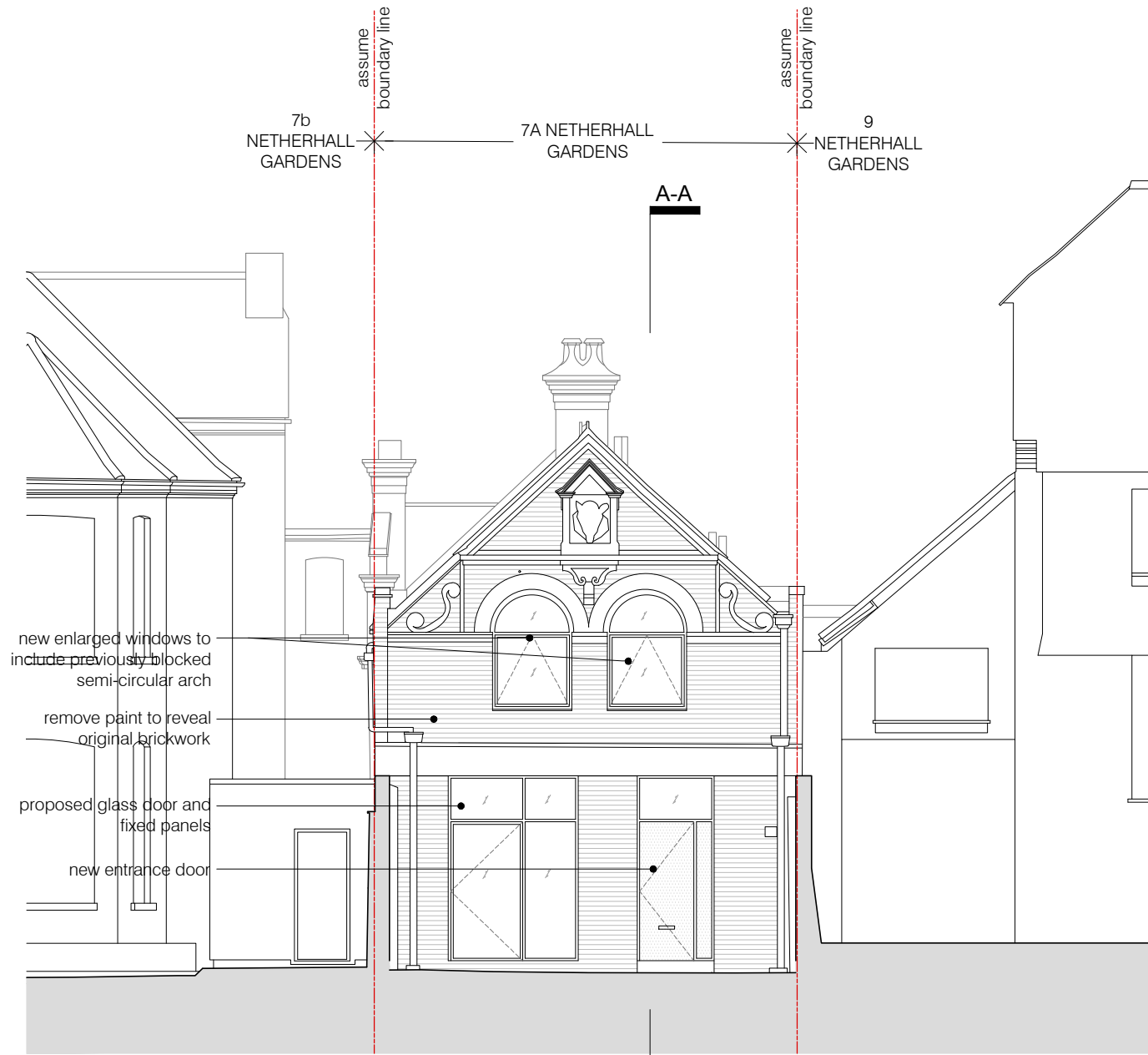
01 PROPOSED FRONT ELEVATION scale 1:100
