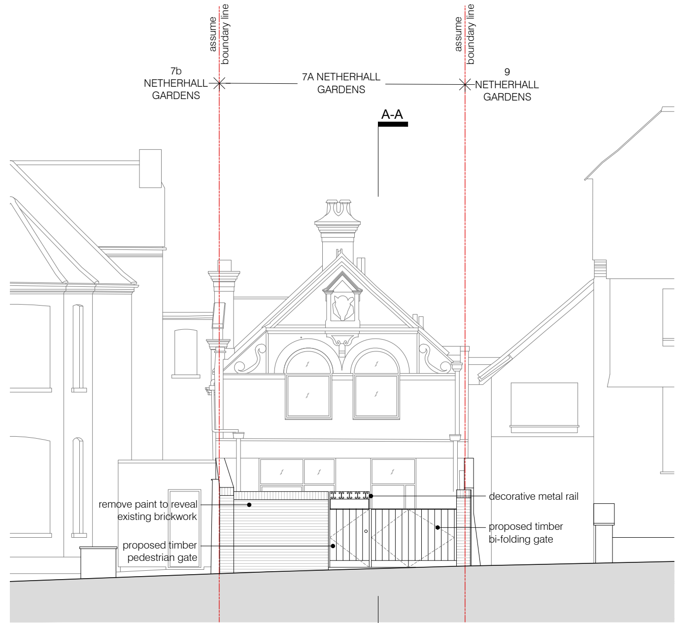
02 PROPOSED STREET ELEVATION scale 1:100
